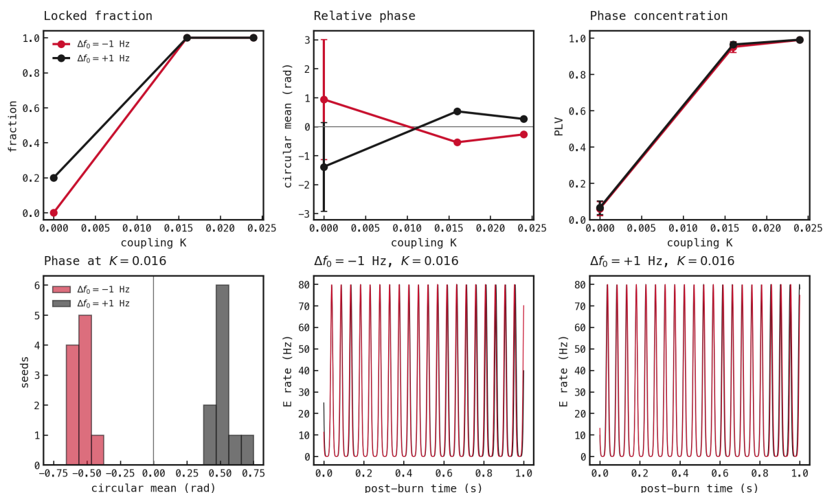
Figure 124: Focused 800 E / 200 I finite-size confirmation. Top panels show locked fraction, circular mean relative phase in radians, and PLV R from Eq. (3) over coupling K for mirrored natural detunings; error bars are one standard deviation across 10 paired seeds. The lower-left panel isolates phase at the disputed coupling. The remaining panels show post-burn E-population rates in hertz (circuit A black, circuit B red). Both detuning signs lock with mirrored phase ordering, resolving the lone 80 E / 20 I exception.
