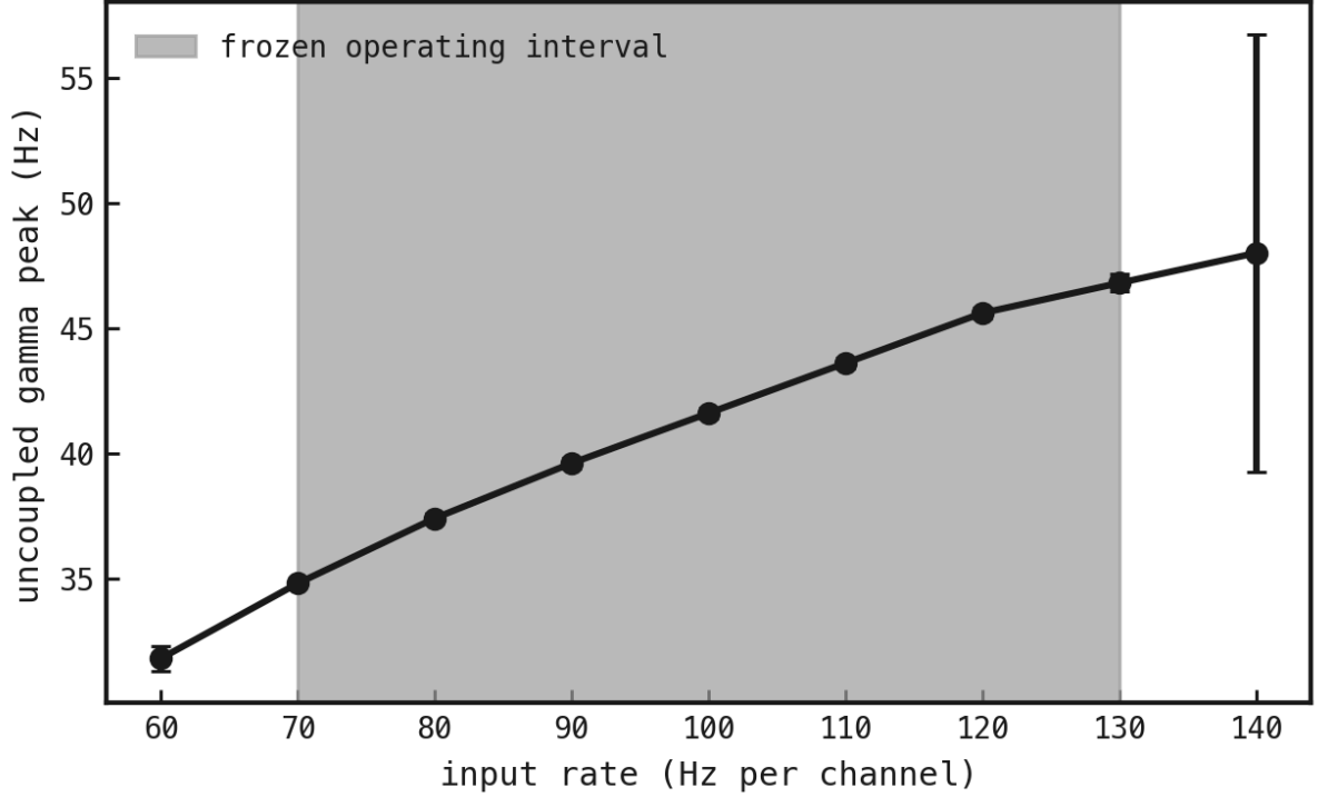
Figure 120: Uncoupled input-rate calibration. Input rate in hertz per channel is on the horizontal axis; median uncoupled gamma peak frequency in hertz is on the vertical axis; bars show half the within-rate interquartile range. The shaded 70–130 Hz interval supplies Eq. (1). The lowest-rate point exceeds the registered within-rate IQR ceiling. At the highest rate, the estimator hops between two separated spectral modes across seeds, producing the large bar. Both boundary conditions are excluded.
