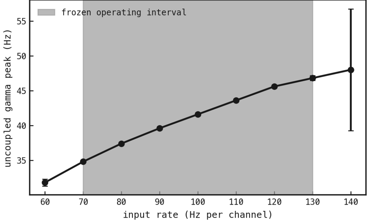
Figure 2: Uncoupled input-rate calibration. Input rate in hertz per channel is on the horizontal axis; median uncoupled gamma peak frequency in hertz is on the vertical axis; bars show half the within-rate interquartile range. The shaded 70–130 Hz interval supplies Eq. (1). The lowest-rate point exceeds the registered within-rate IQR ceiling. At the highest rate, the estimator hops between two separated spectral modes across seeds, producing the large bar. Both boundary conditions are excluded.
