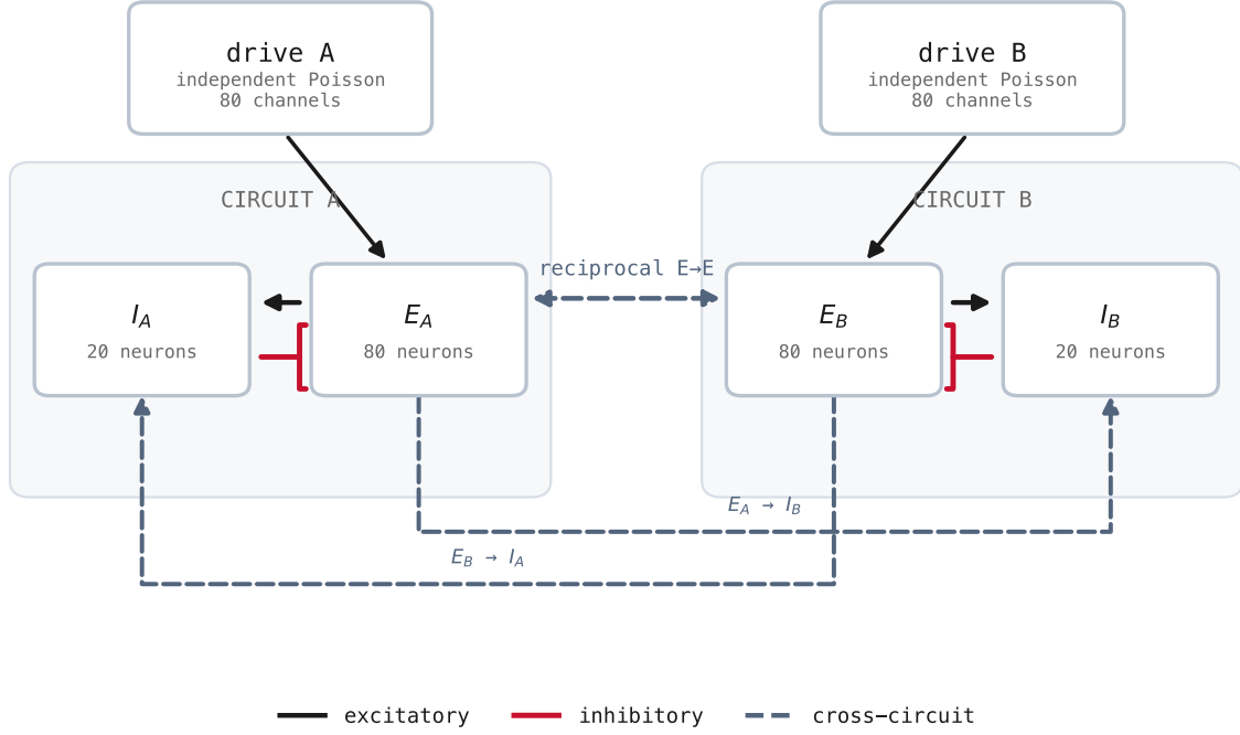
Figure 119: Network graph for the reproduction. Each independent input drives one local E \leftrightarrow I PING loop. Dashed projections are the four reciprocal cross-circuit AMPA pathways varied together by K . Red bar-headed projections are local GABA-A inhibition.
