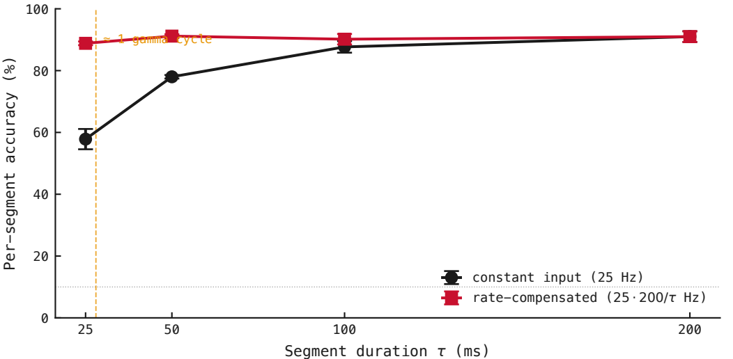
Streaming accuracy vs digit duration on trained PING
