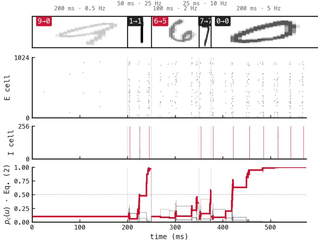
Figure 113: A five-digit variable stream using a variable-rate-trained PING network and its native output-LIF spike-count readout. Counts reset at each boundary while hidden PING state remains continuous. Thumbnail opacity increases with encoding rate; badges show true label and prediction.
