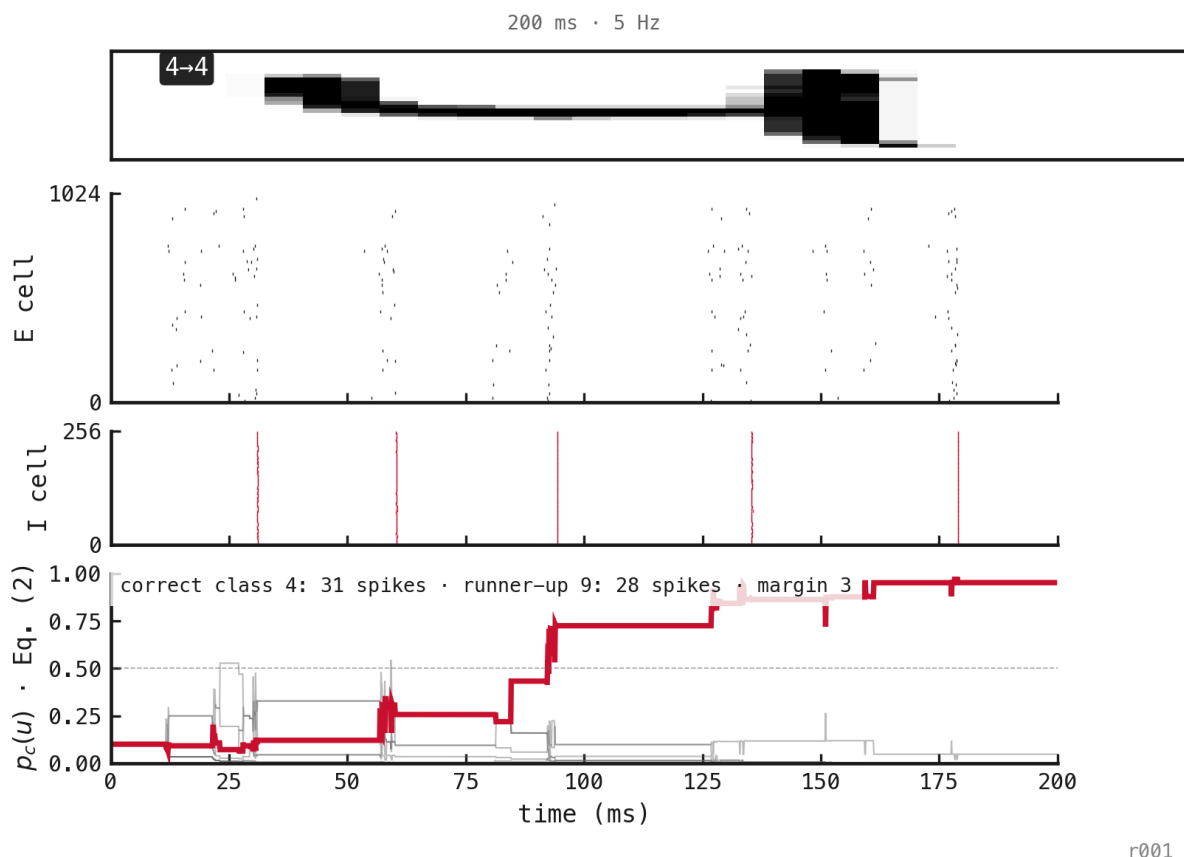
Figure 111: A correctly classified 200 ms presentation at 5 Hz, selected as the first success in a pre-existing matched stream. The result explains the readout trajectory but is not an accuracy estimate. The true and winning class is red.
