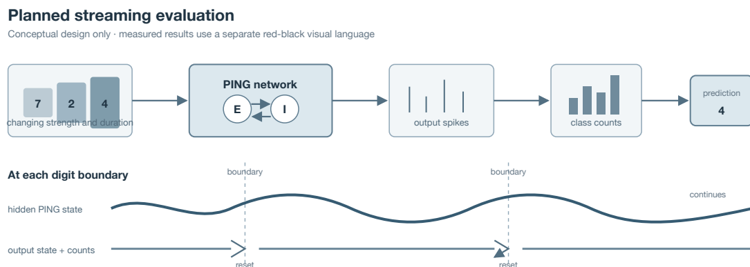
Figure 111: Planned streaming evaluation. Hidden network state continues across digits, while output evidence resets at each boundary. This blue-grey schematic defines the prospective mechanism and is not measured evidence.
