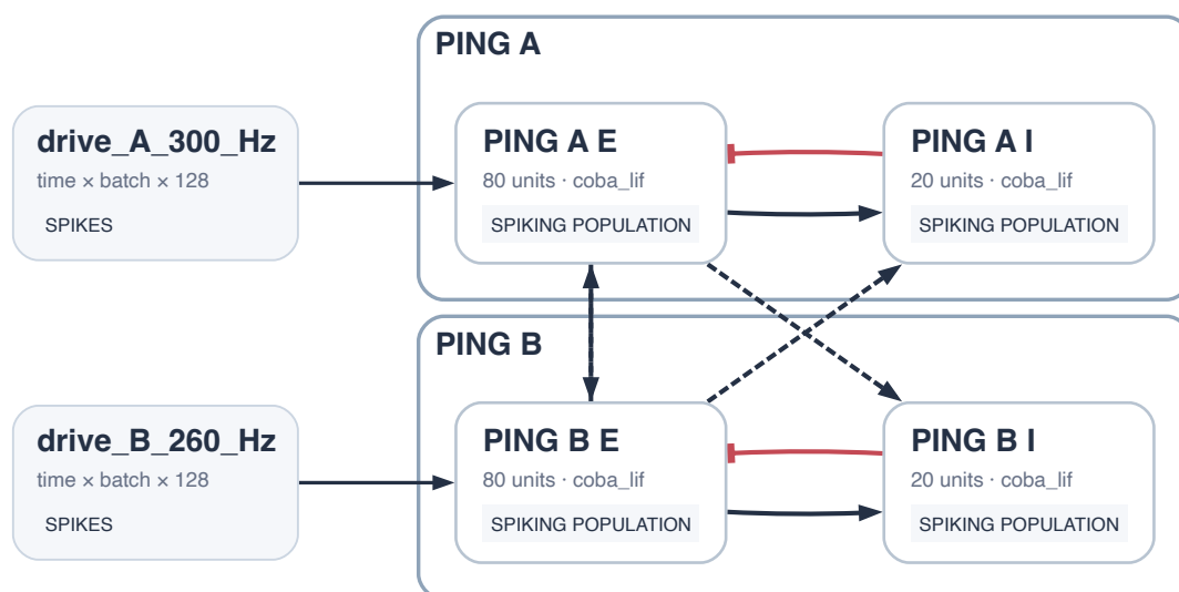
Figure 129: Implemented topology. Networks A and B each contain a local E-to-I-to-E PING loop. Reciprocal projections target E and I populations with independently controlled strengths.
