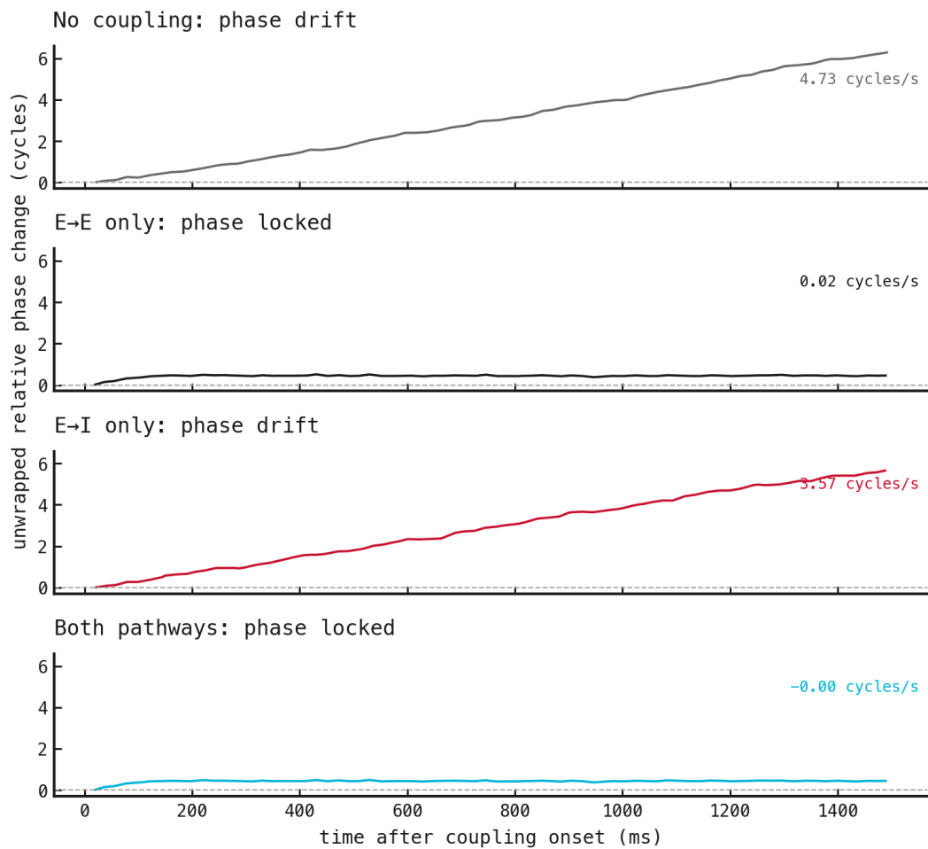
Figure 127: A slope means continued drift; a plateau means phase locking.
