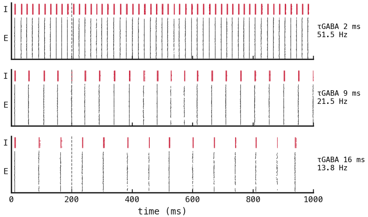
Figure 122: Single paired-trial E and I rasters at the preselected fast, default, and slow inhibitory decay conditions. Time is in milliseconds; E cells are black, I cells are red, and the dashed vertical line marks the transient exclusion. Right labels give inhibitory decay and the resolved dominant frequency.
