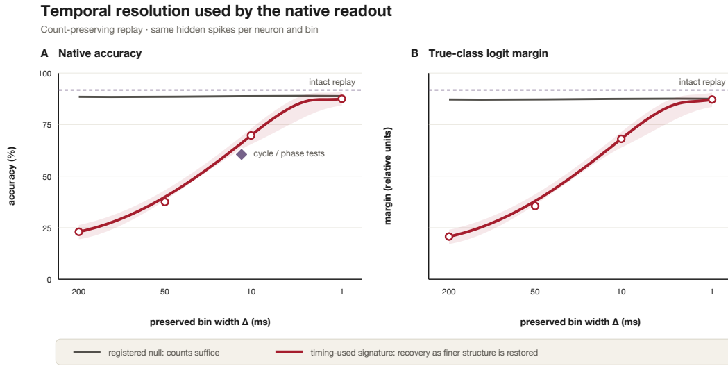
Figure 146: Design schematic for native use. A flat trace means presentation counts suffice. A low coarse-resolution score that recovers toward intact replay as \Delta narrows means the trained output depends on timing at the recovery scale.
