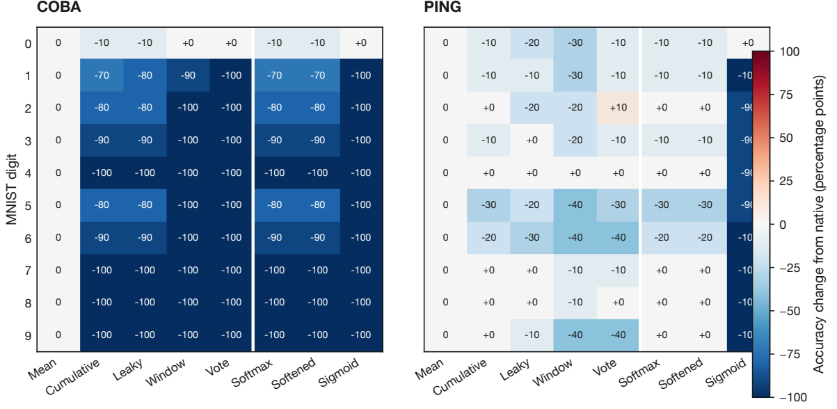
Figure 144: Class-specific changes show whether aggregate loss is confined to one digit.
