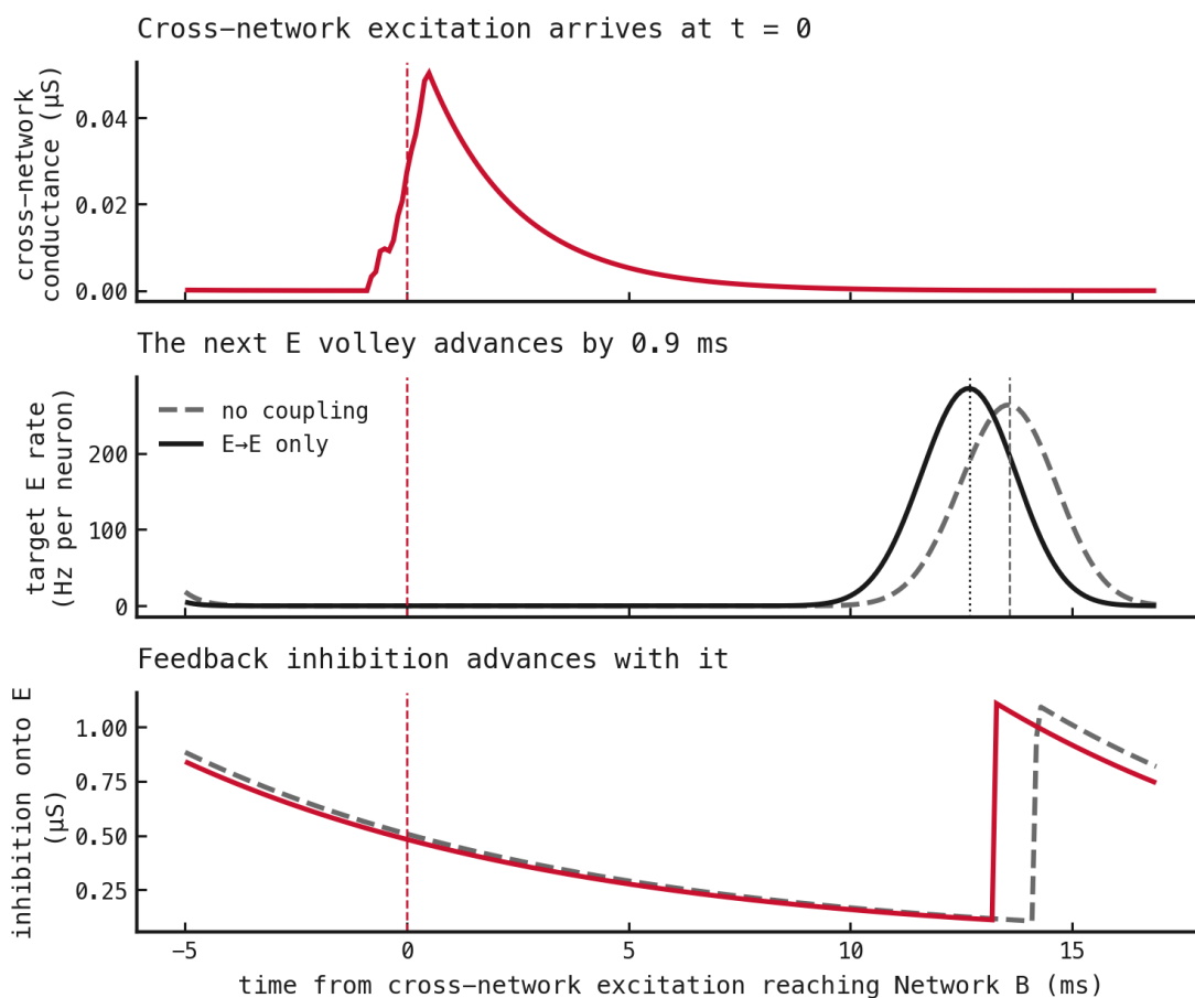
Figure 128: The first correction runs from arriving excitation to an advanced E volley and then advanced feedback inhibition.
