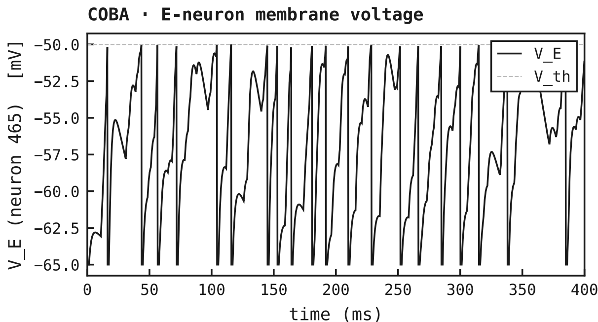
Figure 36: Membrane voltage V_E (black) of the most active E cell, recurrent loop off (COBA, ei-strength 0). Driven only by feedforward input, the cell charges toward threshold ( V_{th} = -50 mV, faint dashed) and hard-resets to V_{reset} = -65 mV each time it fires — irregular, input-paced spiking with no rhythmic structure. The rhythm-free control for Figure 3a.
