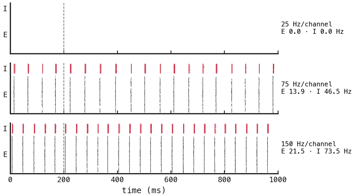
Figure 118: Single-trial E and I rasters at the three input rates fixed before the primary sweep. Time is in milliseconds; E cells are black, I cells are red, and the dashed vertical line marks the 200 ms transient exclusion. The right labels report input rate per channel and post-transient mean population rates in hertz. The 25 Hz condition is silent, whereas the higher-drive conditions show repeated population volleys.
