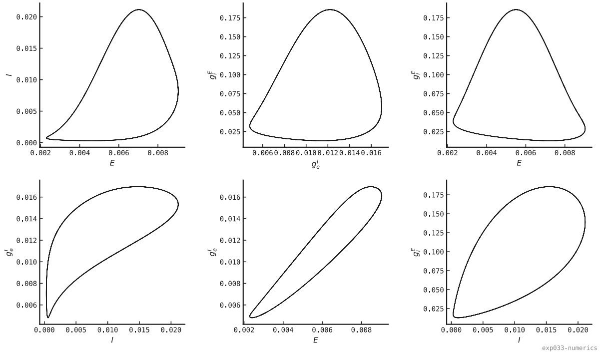
Figure 60: The 4D limit cycle ( I_{\text{ext}} = I^* + 0.4 nA) projected onto all six variable pairs. Every projection is one closed loop: the trajectory lives on a 2D centre manifold. The (E, g_e^I) panel collapses almost to a line: the fast AMPA conductance tracks the E rate, which is why slaving it (the 3D reduction) preserves the dynamics, while the other pairs enclose genuine area and cannot be collapsed.
