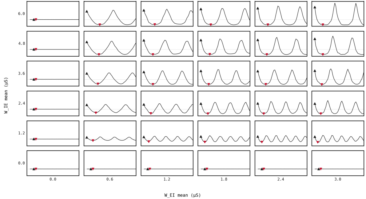
Figure 96: The E-population autocorrelogram A(\ell) for a 6 \times 6 subset of the grid (lag 0–50 ms; dotted line = chance, A = 1 ), with the located lobe ( \blacktriangle ) and trough ( \blacktriangledown ) marked. The two zero edges are flat at 1: asynchronous firing, no structure. Through the interior the Mexican hat emerges: a sharp central lobe at \approx 1 ms over a trough near the half-period, with a secondary peak at the full period further out. The contrast in Figure 1 is exactly this lobe-versus-trough read off as one number.
