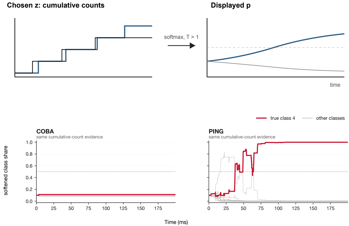
Figure 140: Temperature softening exposes competitors while preserving the winner.
