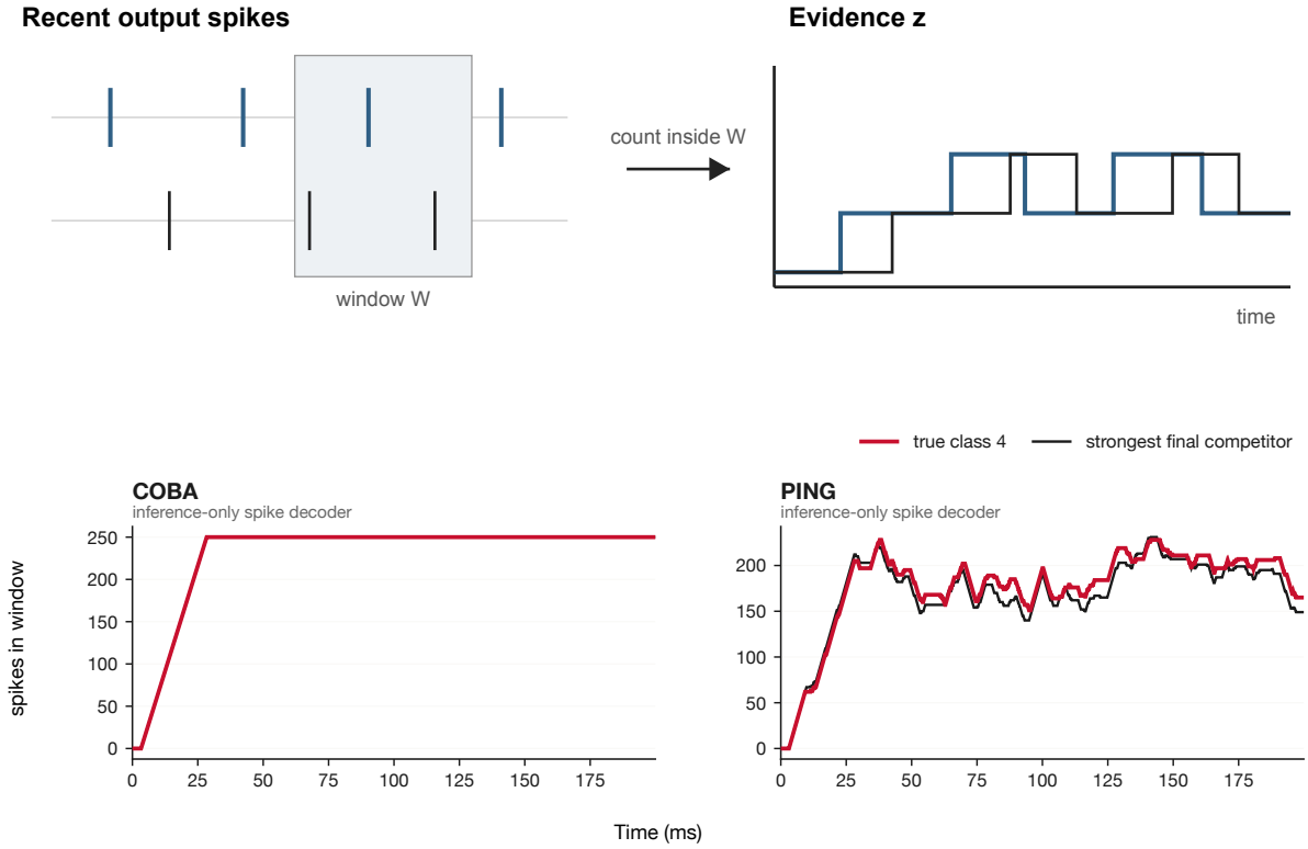
Figure 137: Windowed evidence retains spikes for 25 ms, then removes them.
