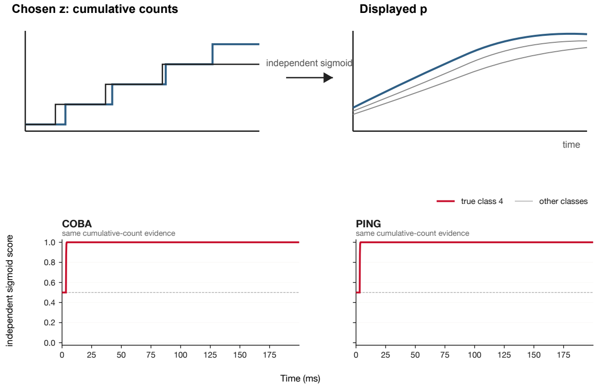
Figure 141: Independent sigmoid bounds each class separately and removes mutual competition.
