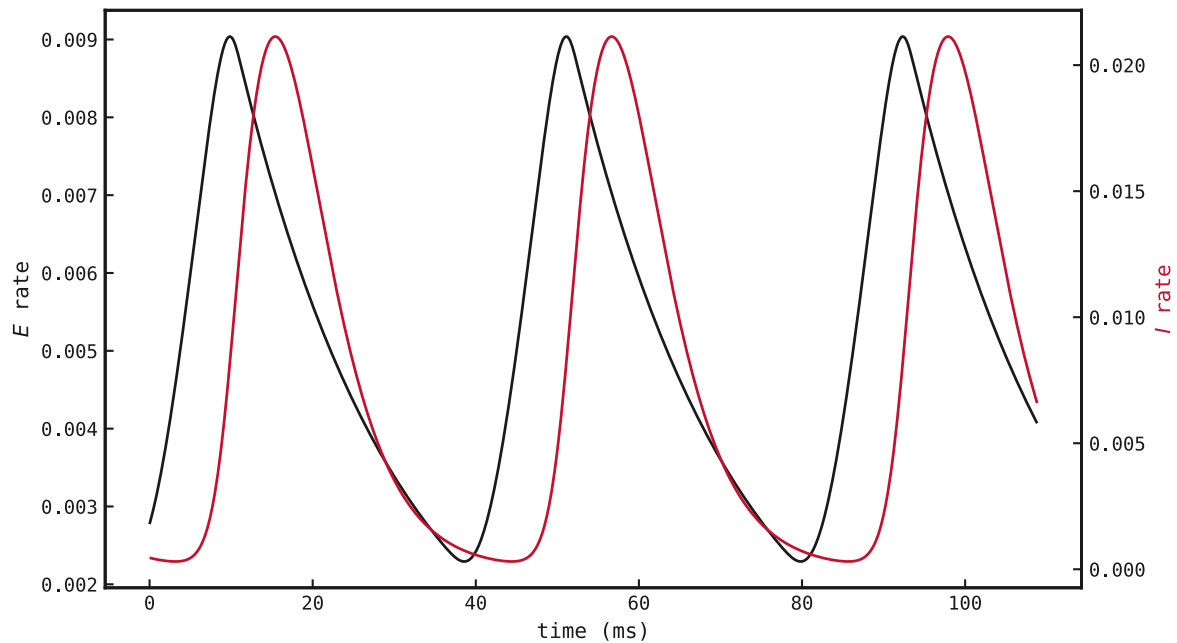
Figure 58: E (black) and I (red) over the limit cycle at I_{\text{ext}} = I^* + 0.4 nA. The E burst leads the I burst by \approx 5.2 ms: E recruits I , I shunts E a few milliseconds later, and the cycle repeats, the loop delay the 2D reduction omits.
