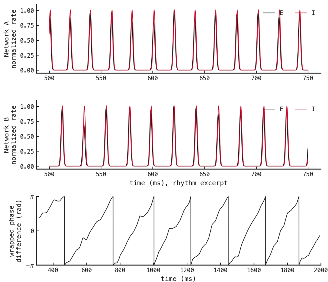
Figure 124: Both networks sustain gamma rhythms, but their relative phase keeps moving. Network A oscillates at 50.7 Hz and Network B at 46.7 Hz. Their low interval variability confirms regular rhythms. Relative phase wraps 7 times, establishing the drift that coupling must stop.
