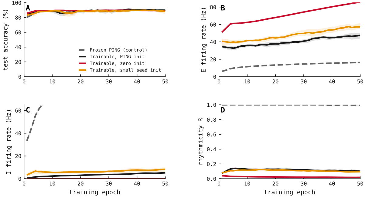
Figure 17: Releasing the loop weights to gradient descent prunes the rhythm within a single epoch, from every initialisation. Per-epoch training metrics with the recurrent weights W^{EI} , W^{IE} made trainable under the Dale’s-law clamp, over 50 epochs on MNIST. Lines are the mean of three seeds (42–44); shading is the across-seed range. Conditions differ only in initialisation of the loop weights: canonical PING values (black), zero (red), and 0.1 \times canonical (amber), against a frozen-PING control (grey, dashed). (A) Test accuracy: all conditions overlap at \approx 84 – 91\% . (B) Mean excitatory firing rate: the trainable conditions rise to \approx 49 – 88 Hz as the loop is dismantled, while the frozen control remains gated near 17 Hz. (C) Mean inhibitory firing rate: the trainable conditions collapse to \approx 0 Hz within a few epochs, while the frozen control’s inhibitory rate rises to \approx 108 Hz as its readout trains. (D) Lobe–trough rhythmicity contrast: the frozen control holds at \approx 1 while every trainable initialisation drains to \approx 0.02 – 0.11 . Source: exp049.
