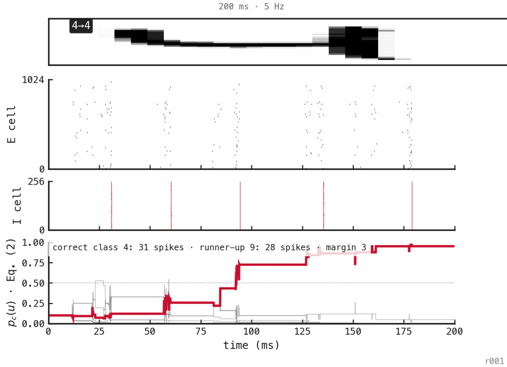
Figure 112: A correctly classified 200 ms presentation at 5 Hz, selected as the first success in a pre-existing matched stream. The figure explains the readout; it does not estimate accuracy. Red marks the true and winning class.
