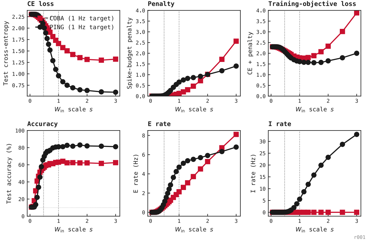
Figure 51: Inference-time W_{in} scale sweep on the two networks trained under the tightest ceiling ( r_{max} = 1 Hz); every W_{in} weight multiplied by a common scalar s , all other weights frozen, 24 values of s \in [0.05, 3] . Top row: CE loss, activity penalty L_{rate} , total objective CE + L_{rate} . Bottom row: test accuracy (chance dotted), E rate, I rate. PING black, COBA red. Vertical dashed line at s = 1 marks the trained operating point; dotted line marks \approx f^* , PING's recruitment cliff. Loss panels clipped at 4; COBA's penalty reaches \approx 3 at s = 3 (rate 2 scaling).
