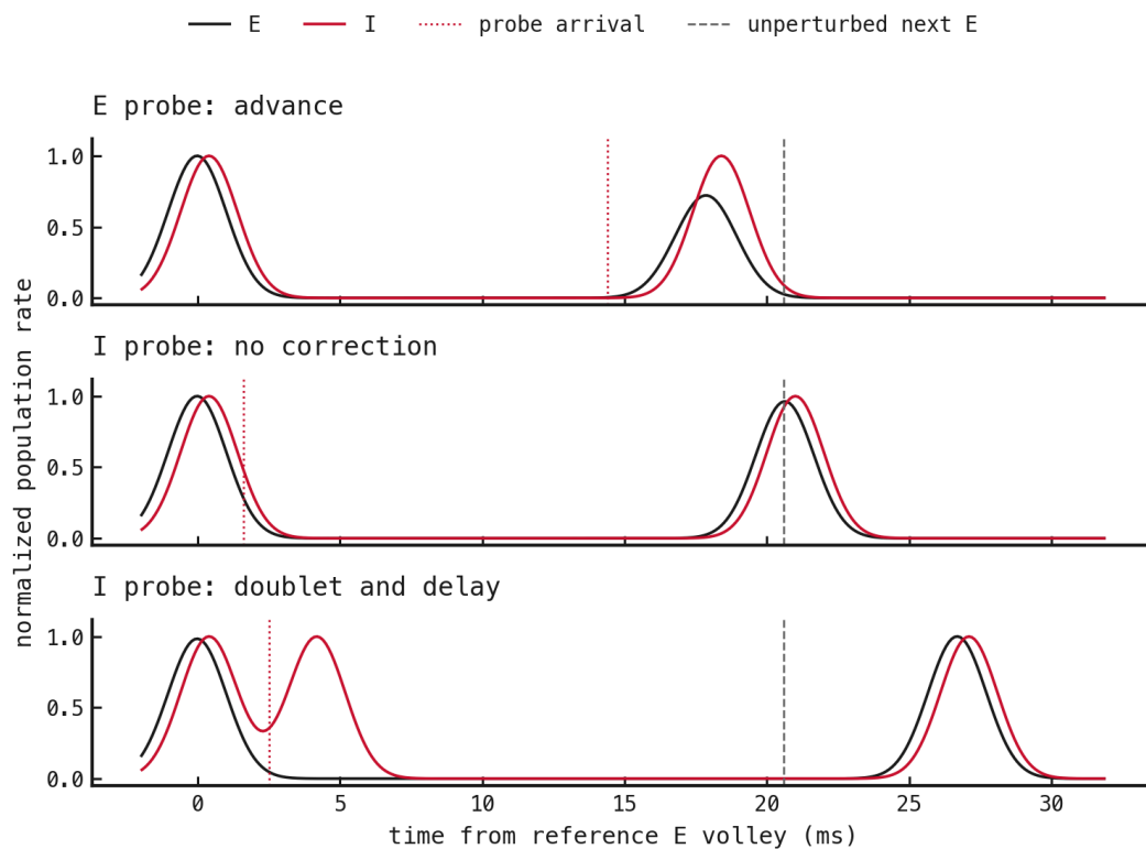
Figure 125: Three representative responses: direct advance, no correction, and doublet-mediated delay.
