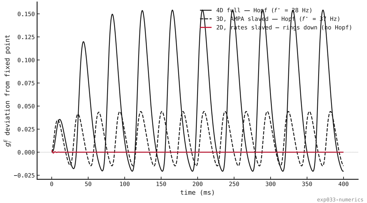
Figure 61: The reductions tested by simulation: g_e^F after a small kick at a common drive ( I_{\text{ext}} = 1 nA, above every threshold). The 4D model (black, f^* = 28 Hz) and the 3D AMPA-slaved reduction (black dashed, f^* = 37 Hz) both sustain the limit cycle; the 2D rate-slaved reduction (red) rings down to its fixed point: no Hopf, as eq (35) requires.
