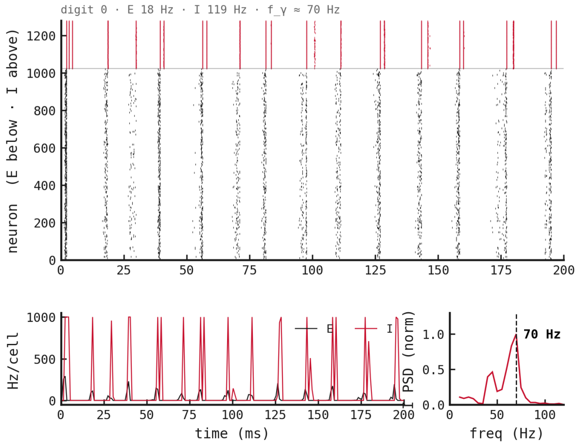
Figure 30: Sample raster: PING at \tau_{\text{GABA}} = 6 ms, seed 42.
