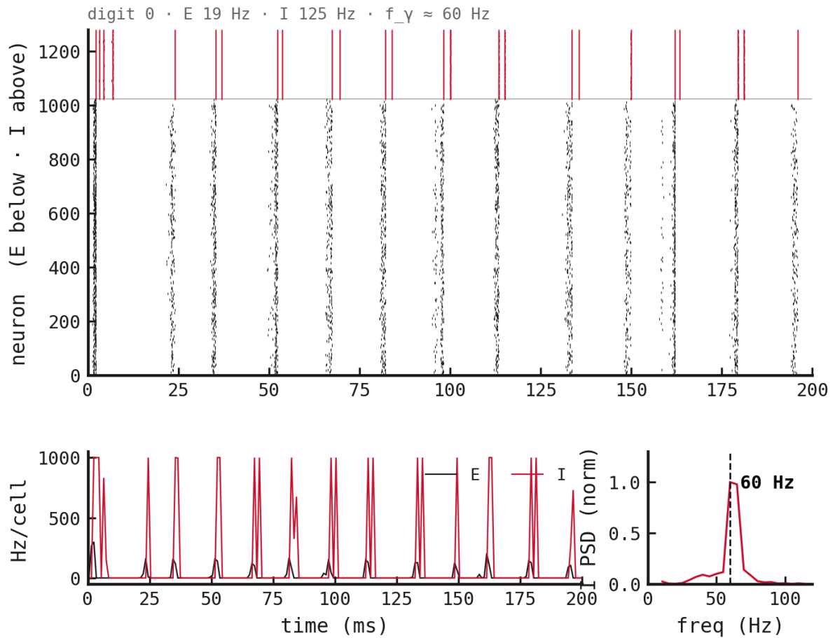
Figure 34: Sample raster: frozen PING recurrent loop, seed 42.
