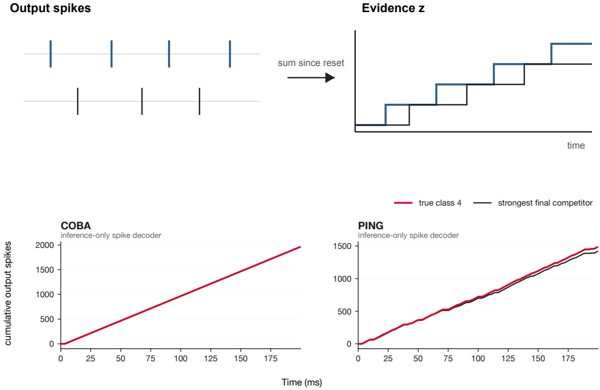
Figure 135: Cumulative evidence preserves every output spike until reset.
