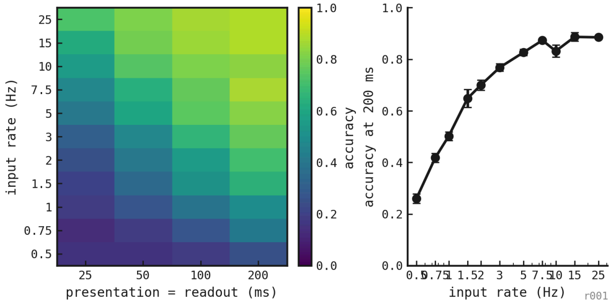
Figure 114: Held-out accuracy across matched presentation/readout durations and trained input rates. The right panel fixes duration at 200 ms to separate rate tolerance from integration time.
