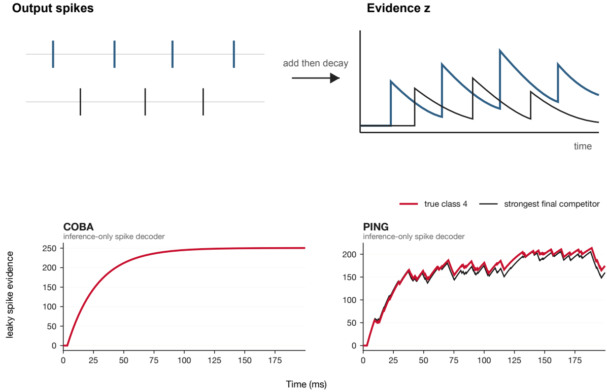
Figure 136: Leaky evidence weights recent output spikes more strongly.
