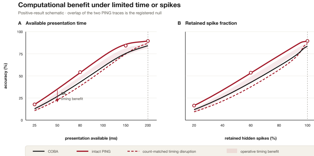
Figure 147: Design schematic for computational benefit. The illustrated positive interaction is a gap between intact and timing-disrupted PING when time or spikes are scarce, followed by convergence when resources are ample. Overlapping PING traces are the registered null.
