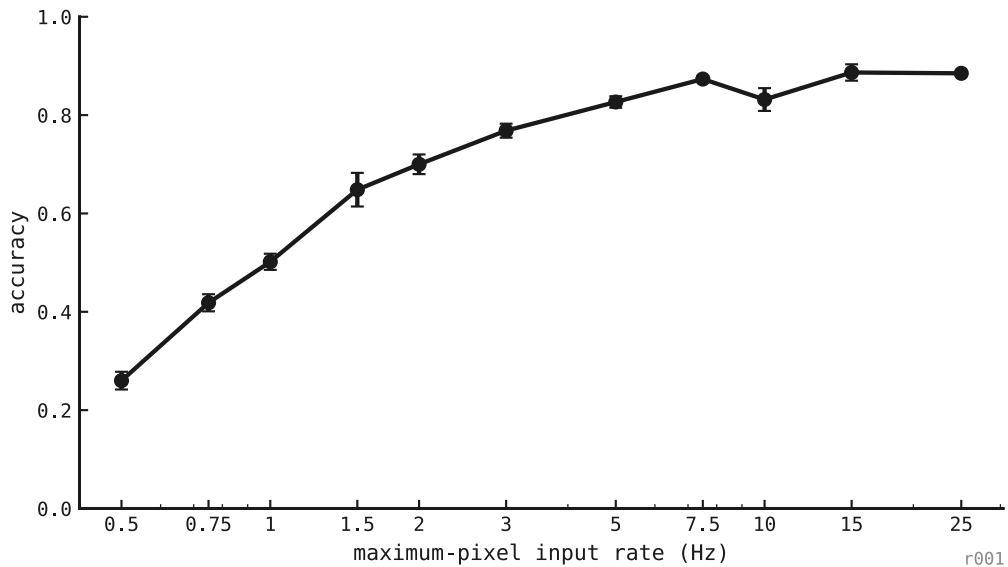
Figure 115: Input-rate psychometric with presentation and spike-count window fixed at 200 ms. Each rate contains 200 held-out digit presentations for each of three trained seeds.
