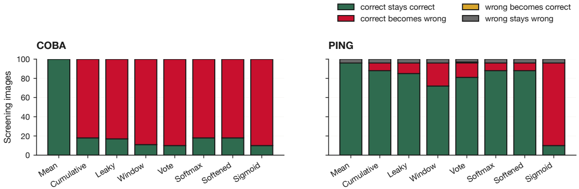
Figure 143: Transitions show whether each alternative preserves, breaks, repairs, or retains a native error.
