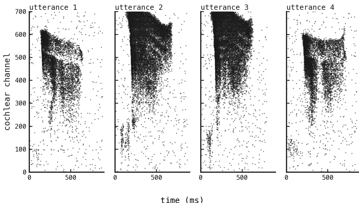
Figure 101: 4 different utterances of class 0, null , each a raster of time (ms) against cochlear channel: the within-class spread. What we expect. Different speakers saying the same word should share a family resemblance while differing in the particulars. What we see. Exactly that: all 4 carry the same broad high-channel onset falling into a mid-channel body, but they differ in duration, event density, and the fine structure of the low-channel tail. This speaker variability is what a classifier trained on SHD must generalise over.
