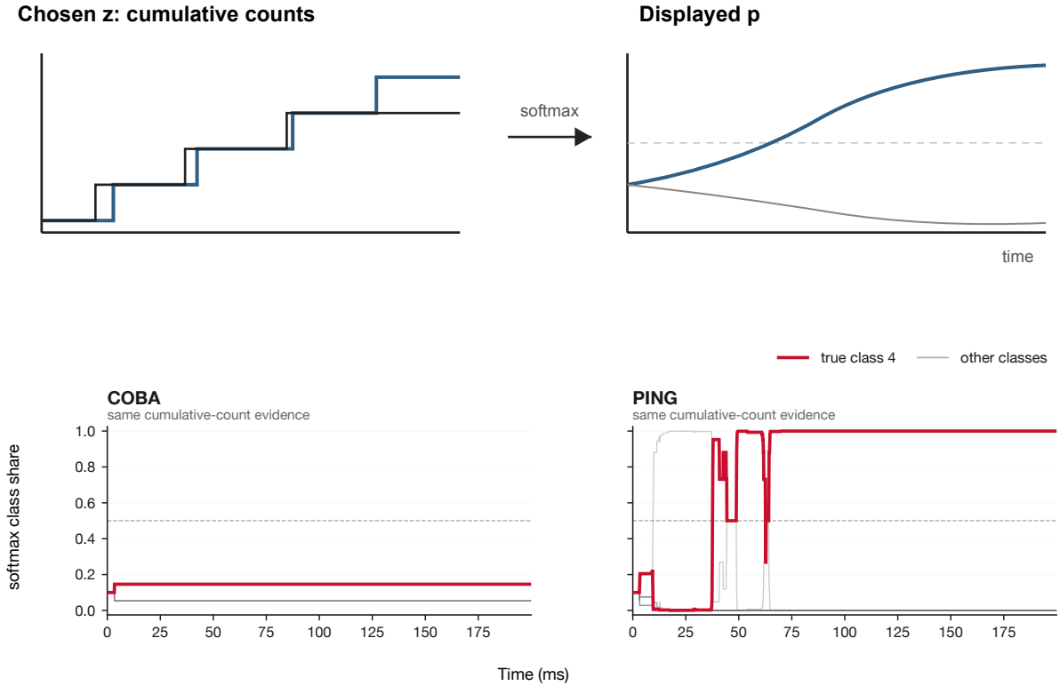
Figure 139: Ordinary softmax converts count margins into competing class shares.
