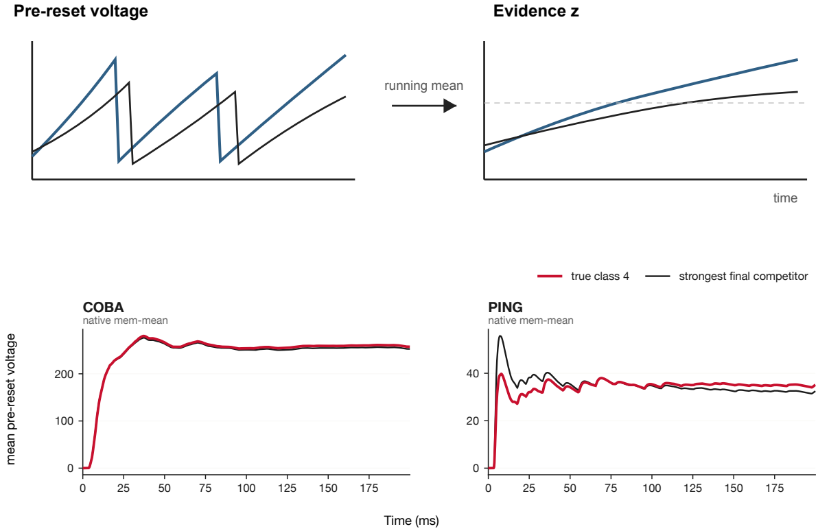
Figure 134: Native mean-voltage evidence retains subthreshold activity while removing temporal order.
