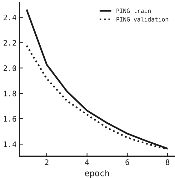
cross-entropy loss
