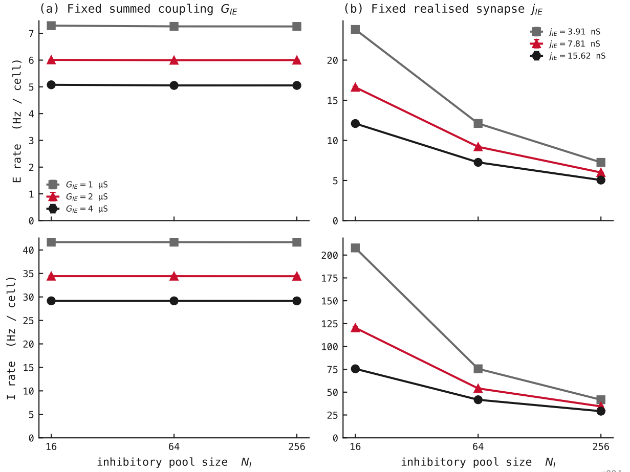
Figure 70: Excitatory and inhibitory firing rates across inhibitory-pool size under two I \rightarrow E scaling controls. Top: excitatory-cell rate in Hz per cell. Bottom: inhibitory-cell rate in Hz per cell. (a) Holding the expected summed I \rightarrow E coupling G_{IE} fixed makes the realised synapse j_{IE} = \frac{G_{IE}}{N_I} shrink as the pool grows. (b) Holding j_{IE} fixed makes summed coupling grow with N_I . Each curve is one coupling level; markers are means and error bars \pm 1 standard deviation (SD) over 3 seeds, with 8 trials per seed. The controls coincide at the reference pool N_I = 256 . Rates are invariant to pool size only under inverse scaling of individual synapses.
