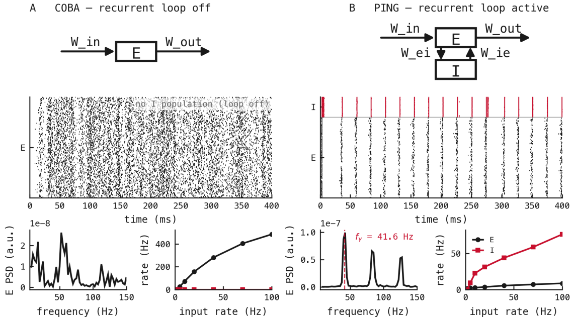
Figure 23: The architecture and its behaviour, off and on, on the same network. Each column carries its schematic on top — A COBA (input→ E →output, no I population) and B PING (the same plus the recurrent E \leftrightarrow I loop, W_{ei} down and W_{ie} up) — directly above the plots it produces. Below each schematic is one combined raster ( E black in the lower portion, I red in the upper portion — same axes, no gap) above a bottom row pairing the Welch PSD of the population-mean E trace with the free-running f - I curve (mean per-cell rate vs input rate, E black / I red; each column has its own y-axis — COBA runs to its \approx 400 + Hz ceiling, PING is on a smaller scale so its loop-clamped E and climbing I are legible). Rasters and spectra are on uniform Poisson input (400 ms) at per-condition rates (COBA 5 Hz, PING 45 Hz — see Methods); the f - I curves sweep that drive on the untrained network. All runs are at \Delta t = 0.1 ms. A — COBA ( ei-strength 0, loop off): asynchronous E firing, no I activity, no recurrent gamma peak, and an E f - I curve that climbs steeply with input rate and saturates toward the refractory ceiling. B — PING ( ei-strength 1.5, loop on): the I population fires a synchronous burst once per cycle and the E raster breaks into vertical bands (the I volley trails each E volley by the AMPA delay); the PSD carries a clean gamma peak (dashed red line; f_\gamma measured from this raster’s E -population PSD, marked on the plot); and its f - I shows the E rate held to single digits across the whole sweep (note the much smaller y-axis than COBA’s) while inhibition climbs — the loop’s dynamic-range compression. The single E \rightarrow I \rightarrow E loop is the only change: it converts asynchronous firing into a gamma rhythm and clamps the E rate.
