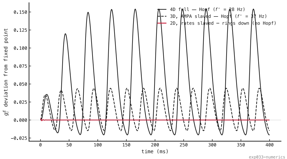
Figure 49: The reductions tested by simulation: g_f^E after a small kick at a common drive ( I_{\text{ext}} = 1 nA, above every threshold). The 4D model (black, f^* = 28 Hz) and the 3D AMPA-slaved reduction (black dashed, f^* = 37 Hz) both sustain the limit cycle; the 2D rate-slaved reduction (red) rings down to its fixed point: no Hopf, as eq (35) requires.
