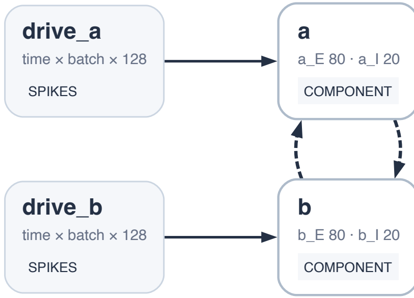
Figure 106: Proposed SNNLANG graph. Each PING network contains 80 excitatory and 20 inhibitory cells. The dashed reciprocal links contain four AMPA projections. Their shared weight is K = 0 before coupling and K = 0.08 after coupling.
