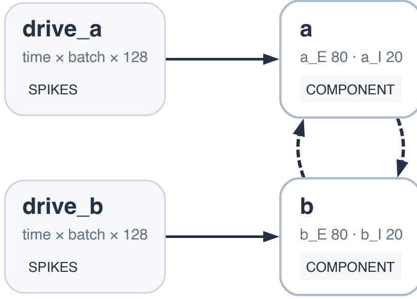
Figure 1: Proposed SNNLANG graph. Each PING network contains 80 excitatory and 20 inhibitory cells. The dashed reciprocal links contain four AMPA projections. Their shared weight is K = 0 before coupling and K = 0.08 after coupling.
