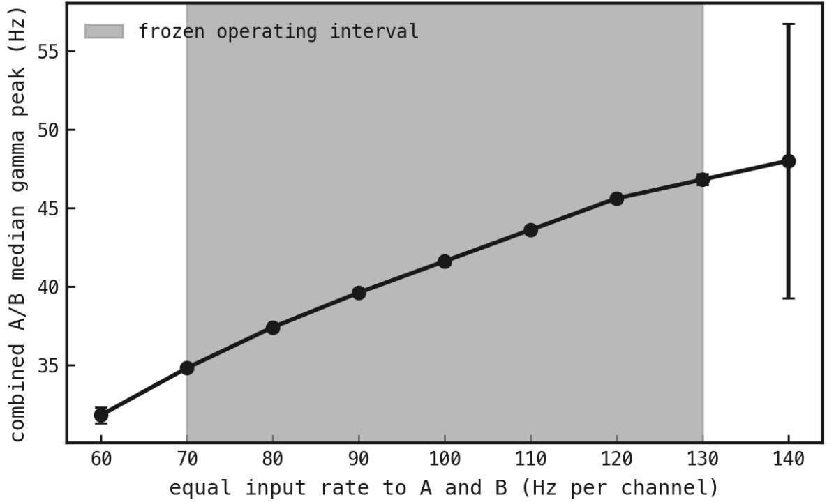
Figure 120: Uncoupled input-rate calibration. Circuits A and B receive the same input rate, shown in hertz per channel on the horizontal axis. At each rate, the vertical coordinate is the median of 10 gamma-peak estimates: both circuits from each of five trials. Bars show half the interquartile range of the combined A and B estimates, spanning the middle half of the data. The shaded 70–130 Hz interval supplies Equation 1. The lowest-rate point exceeds the registered within-rate IQR ceiling. At the highest rate, the estimator hops between two separated spectral modes across seeds, producing the large bar. Both boundary conditions are excluded.
