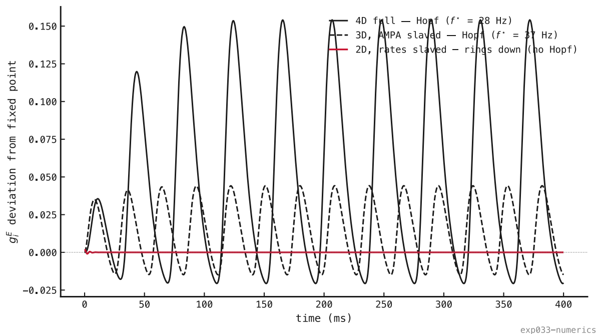
Figure 73: The reductions tested by simulation: g_i^E after a small kick at a common drive ( I_{\text{ext}} = 1 nA, above every threshold). The 4D model (black, f^* = 28 Hz) and the 3D AMPA-slaved reduction (black dashed, f^* = 37 Hz) both sustain the limit cycle; the 2D rate-slaved reduction (red) rings down to its fixed point: no Hopf, as eq (35) requires.
