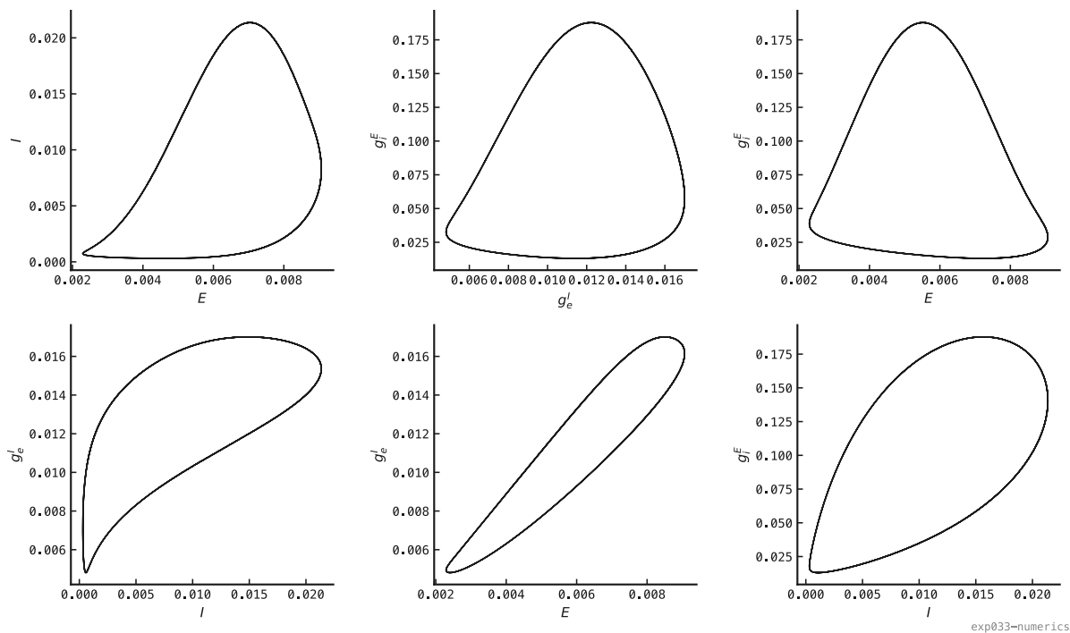
Figure 72: The 4D limit cycle ( I_{\text{ext}} = I^* + 0.4 \text{ nA} ) projected onto all six variable pairs. Every projection is one closed loop: the trajectory lives on a 2D centre manifold. The (E, g_e^I) panel collapses almost to a line: the fast AMPA conductance tracks the E rate, which is why slaving it (the 3D reduction) preserves the dynamics, while the other pairs enclose genuine area and cannot be collapsed.
