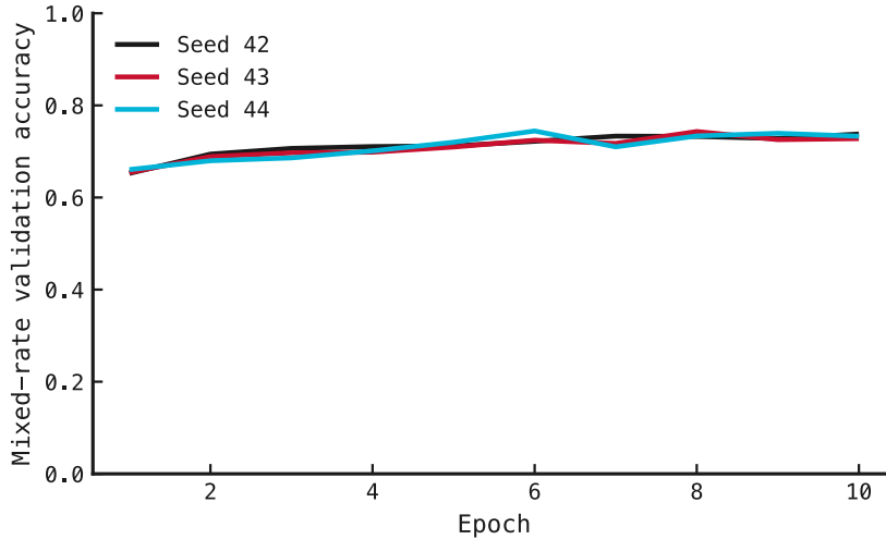
Figure 125: Mixed-rate validation histories for the three independently trained nonlinear decoders. Every epoch used fresh direct feature simulations.
