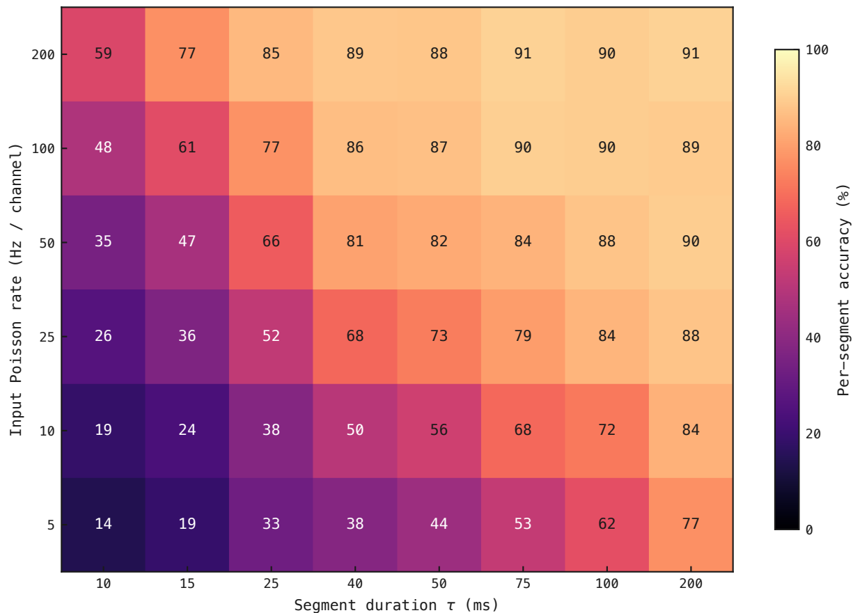
Streaming accuracy across ( \tau , input rate) on trained PING
