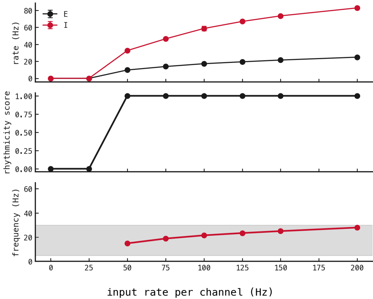
Figure 112: Response of one fixed default PING graph to homogeneous Poisson drive. Top: mean E and I firing rates in hertz, with standard deviations across 5 paired trials. Middle: median lobe-trough rhythmicity contrast R , with error bars showing half the interquartile range; R = 0 is flat and R approaches 1 as periodic structure strengthens. Bottom: median dominant E-population frequency in hertz after subharmonic correction; the grey region marks 5–30 Hz. Rhythmicity switches on abruptly at 50 Hz per channel, while the dominant rhythm increases smoothly from 14.93 Hz.
