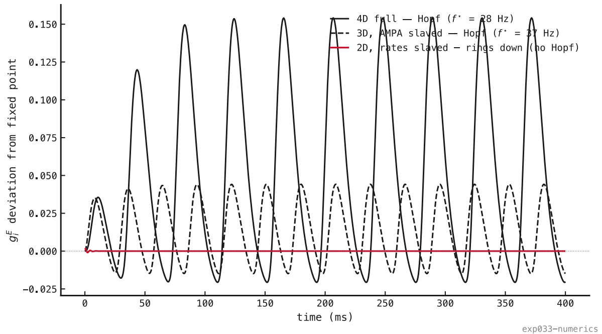
Figure 61: The reductions tested by simulation: g_e^E after a small kick at a common drive ( I_{\text{ext}} = 1 nA, above every threshold). The 4D model (black, f^* = 28 Hz) and the 3D AMPA-slaved reduction (black dashed, f^* = 37 Hz) both sustain the limit cycle; the 2D rate-slaved reduction (red) rings down to its fixed point: no Hopf, as eq (35) requires.
