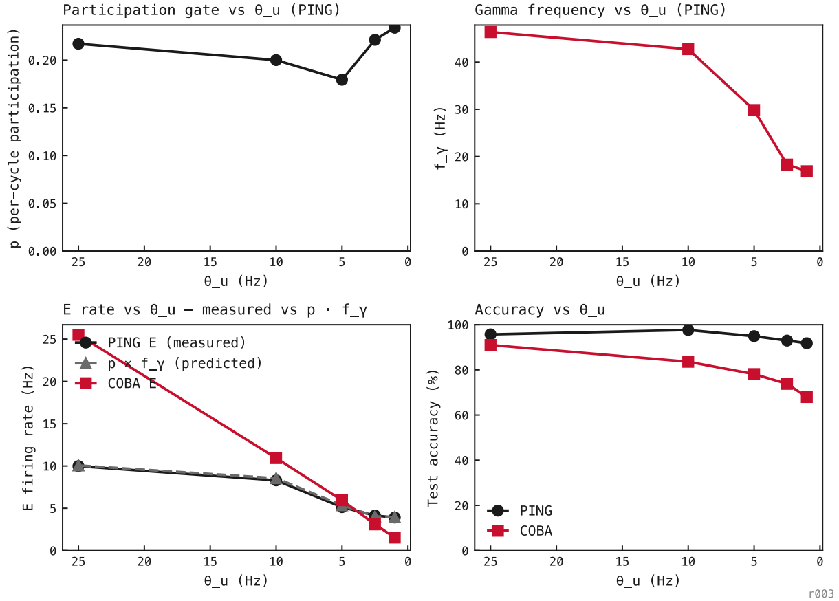
Figure 49: Five representative seed-42 PING rate-target checkpoints, 256 test trials each. p stays in 0.18–0.23 across the entire sweep (the architecture protects the participation gate), while f_\gamma slides from \approx 46 Hz to \approx 17 Hz as the penalty tightens. The grey dashed p \cdot f_\gamma curve overlays the measured E rate within 4%; the rate change is entirely in f_\gamma . PING accuracy holds at 92–98% the whole way; COBA’s collapses from 91% to 68%.
