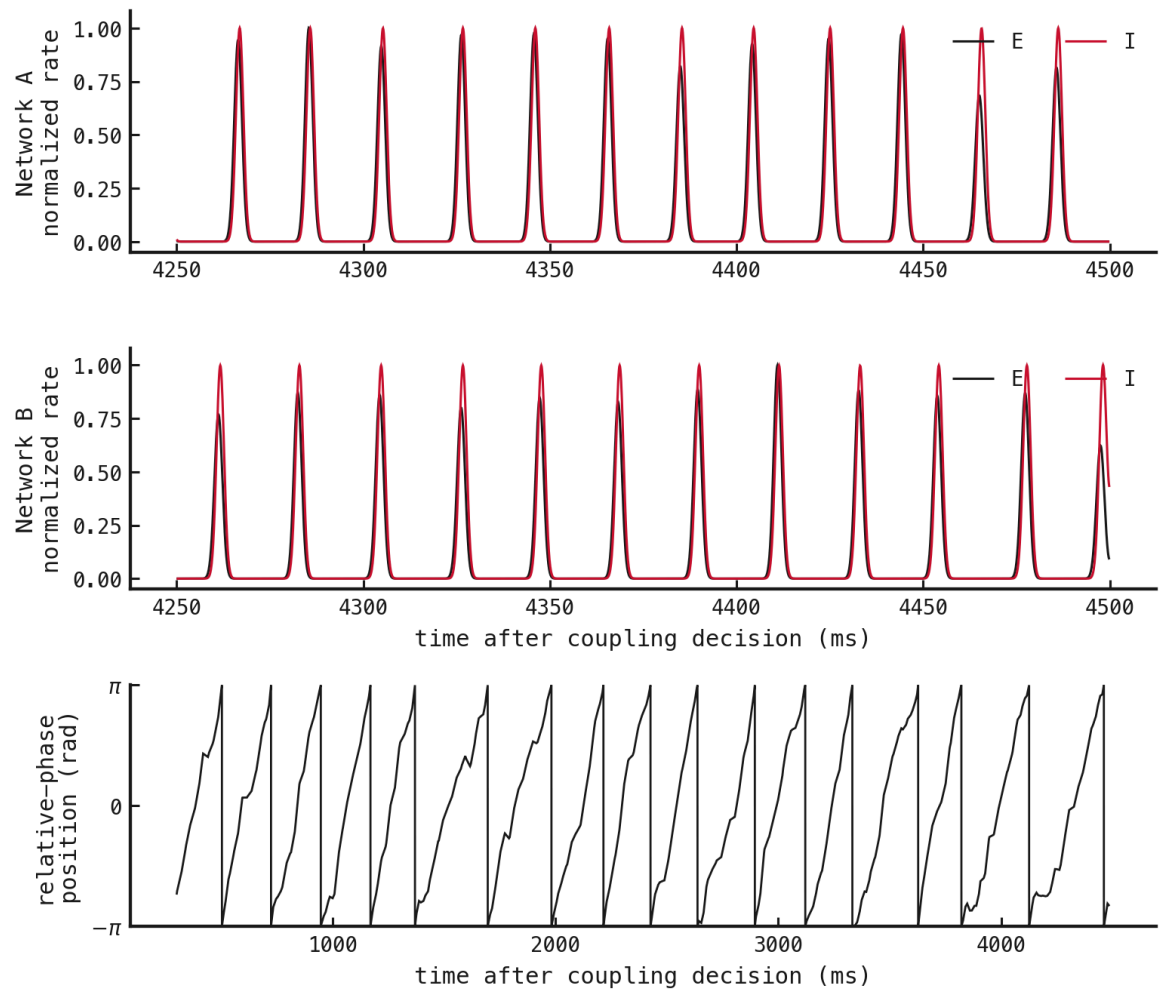
Figure 125: Both uncoupled networks maintain regular PING rhythms, but Network A runs at 50.6 Hz and Network B at 46.6 Hz. Their relative phase therefore circulates, completing 16 slips with phase concentration 0.028.
