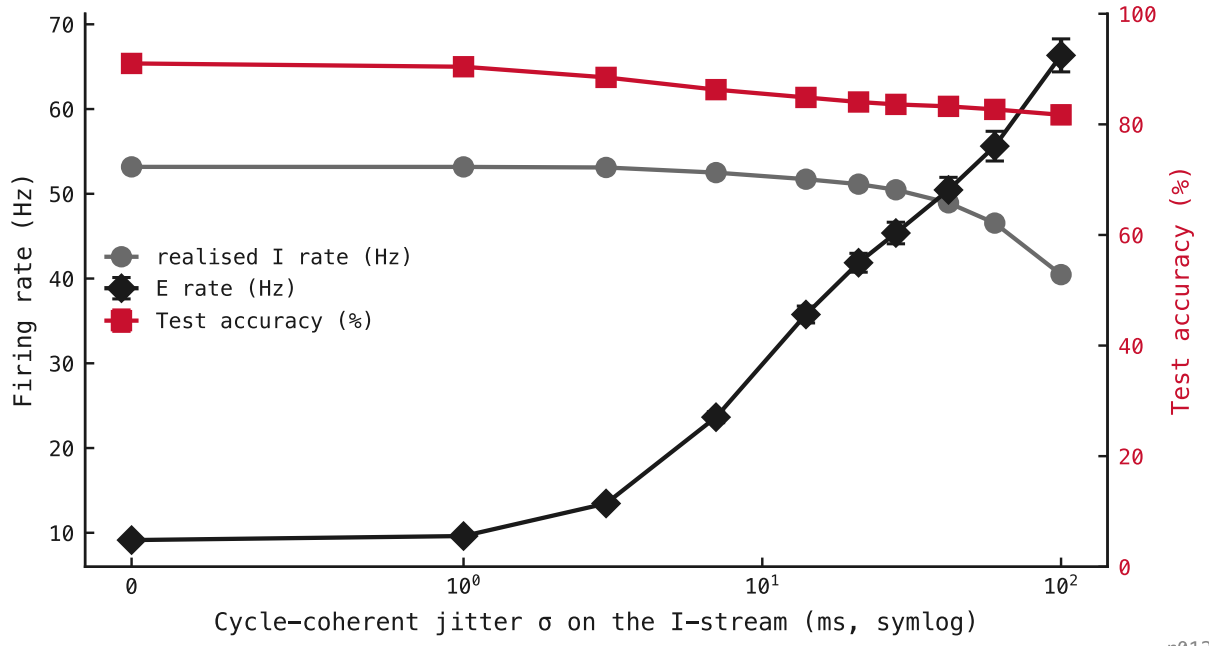
Figure 76: E rate (black diamonds) and accuracy (red squares) vs cycle-coherent jitter \sigma , three seeds. As \sigma grows the displaced bursts open wider gaps and the E rate climbs from baseline (9.1 Hz) past the full phase-shuffle level (25.9 Hz, the reference with within-burst structure destroyed) to 66.3 Hz by \sigma = 100 ms, with the sharpest rise near the predicted transition timescale \sigma = 1/f_\gamma \approx 22.8 ms; accuracy declines only gently, holding near 81.7%. The grey trace is the realised mean I rate: it holds within 3% of baseline through \sigma \approx 14 ms — where the E rate has already risen to 35.8 Hz — then droops to 40.5 Hz (24% below baseline) by \sigma = 100 ms, as the finite trial window truncates the most-displaced bursts. The strict same-mean-inhibition comparison is read at the smaller \sigma , where the rate is matched and the E rise is already unambiguous.
