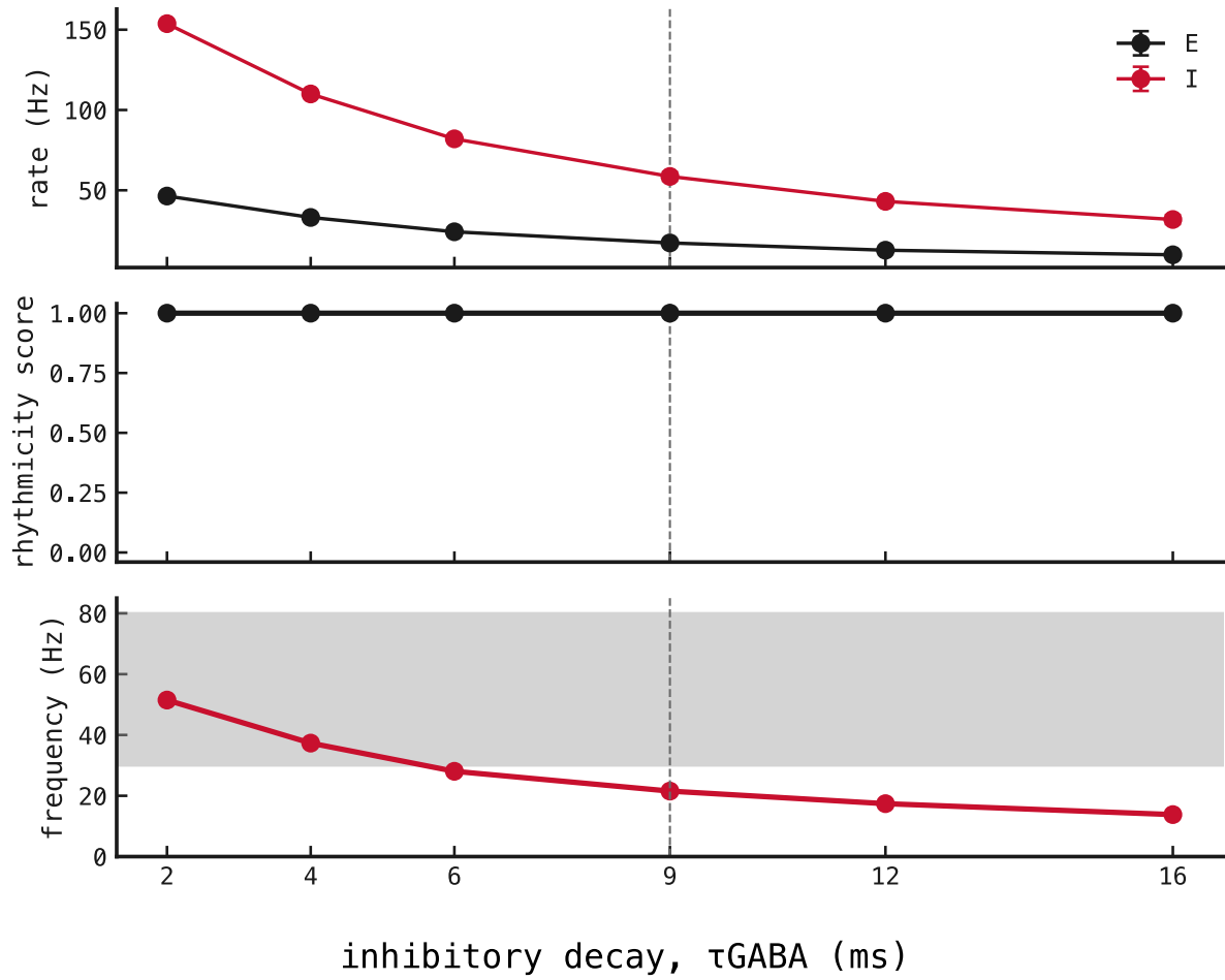
Figure 116: Response to inhibitory synaptic decay at fixed 100 Hz/channel input. Top: mean E and I firing rates with standard deviations across 5 paired trials. Middle: median standard rhythmicity contrast R , with half-interquartile-range error bars. Bottom: median dominant E-population frequency; the grey region marks 30–80 Hz gamma. The dashed line marks the 9 ms component default.
