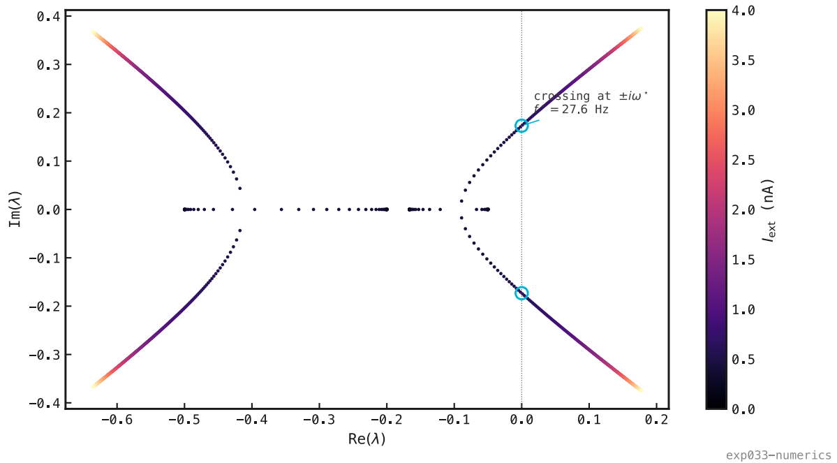
Figure 55: How to read it. Each dot is one eigenvalue \lambda of the Jacobian (28). Its horizontal position is the growth rate \text{Re } \lambda (negative means that mode decays, positive means it grows), and the dotted line at \text{Re } \lambda = 0 is the stability boundary: everything to its left is damped. Its vertical position is the oscillation frequency \text{Im } \lambda (zero = a non-oscillating mode, on the real axis). The Jacobian is 4 \times 4 , so each drive contributes four dots; sweeping I_{\text{ext}} (colour, dark→bright) drags them along the curves shown. Follow the upper and lower arms: one complex-conjugate pair lifts off the real axis and marches rightward, touching the boundary at \pm i\omega^* (cyan circles) when I_{\text{ext}}^* = 0.6 nA. That crossing is the Hopf, where the network tips from damping to amplifying, and the height of the crossing sets the rhythm, f^* = \omega^*/2\pi \approx 27.6 Hz. The other two eigenvalues stay left of the line throughout, so a single oscillation goes unstable: a simple Hopf. (A second pair reaches the axis only at far higher drive, above the recruitment cliff.)
