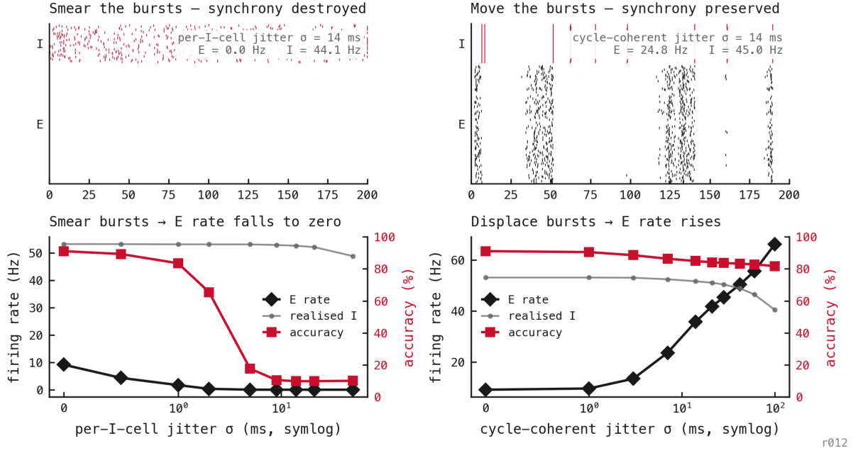
Figure 73: Two inference-time perturbations of the trained-PING I-stream, both holding the mean per-cell I rate fixed at \approx 53.2 Hz , push the E rate in opposite directions, which a mean-inhibition account cannot produce. Both columns use the same jitter magnitude, \sigma = 14 ms — only the kind of jitter differs. Left column, smear the bursts : per-I-cell jitter (realised I 52.5 Hz) scatters the spikes within each burst, destroying synchrony while leaving the mean untouched; the burst dissolves into a continuous shunt, the E rate falls to zero, and accuracy collapses toward chance (9.9% at the Poisson limit). Right column, move the bursts : cycle-coherent jitter (realised I 51.7 Hz — within 3% of the left column) displaces each gamma burst bodily but keeps its within-burst synchrony; the I-stream opens gaps and the E rate rises from 9.1 Hz at baseline to 35.8 Hz, accuracy holding near 84.9%. Same jitter magnitude, same mean inhibition (both \approx 53.2 Hz), opposite outcome: what gates the E rate is the timing of inhibition, the rhythm, not its average level. The cycle-coherent rise continues past the full phase-shuffle level to 66.3 Hz by \sigma = 100 ms (bottom-right sweep), but there the finite trial window truncates the most-displaced bursts and realised I falls 24%, so the strict rate-matched reading is taken at \sigma = 14 ms; see Methods.
