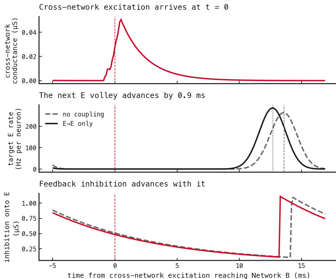
Figure 123: The first correction runs from arriving excitation to an advanced E volley and then advanced feedback inhibition.
