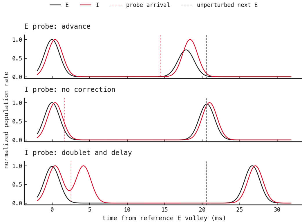
Figure 120: Three representative responses: direct advance, no correction, and doublet-mediated delay.
