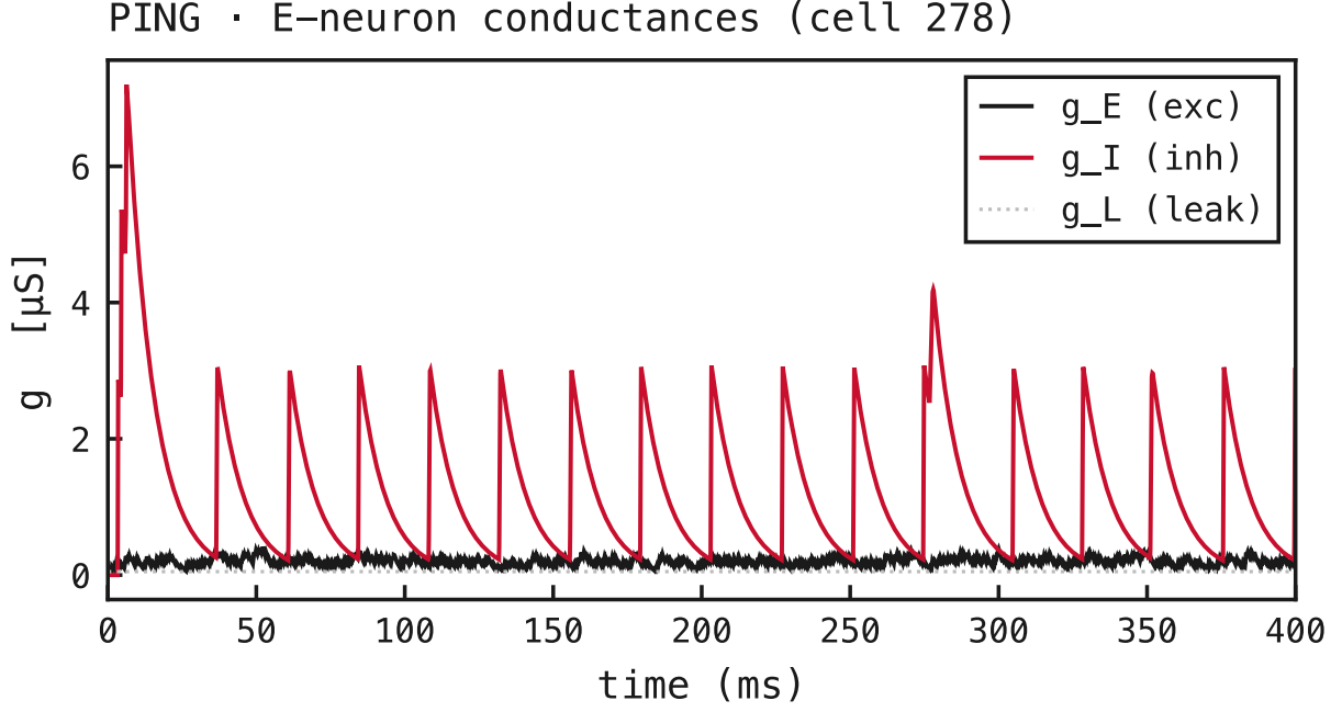
Figure 6: Conductances on the same E cell, PING mode. The inhibitory conductance g_I (red) now dominates — it spikes once per gamma cycle as the synchronous I-burst arrives through W_{ie} , then decays with \tau_{\text{GABA}} — while g_E (black) carries the smaller feedforward input and g_L (faint) is fixed. All three traces are non-negative : g_I is large and positive, and that is what shunts the cell — it carries no sign of its own.
