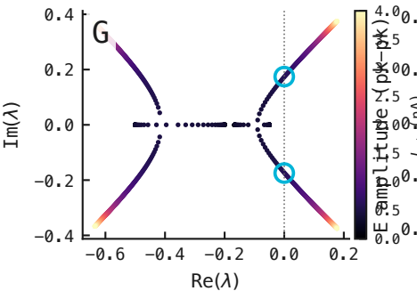
Hopf crossing at I^* = 0.60 nA
