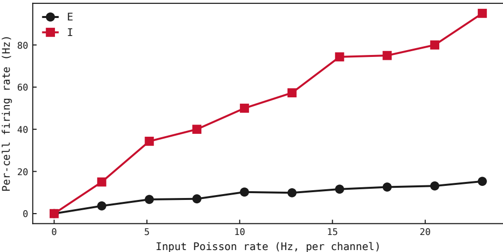
Trained PING f-I curve (MNIST digit 0)
