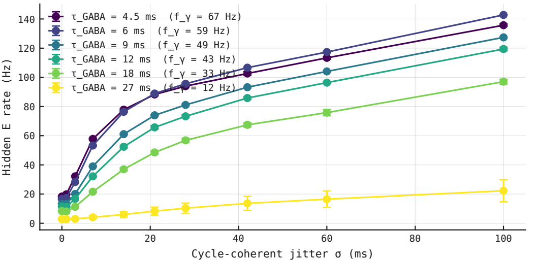
Jitter sweep across \tau_{\text{GABA}} – raw \sigma axis
