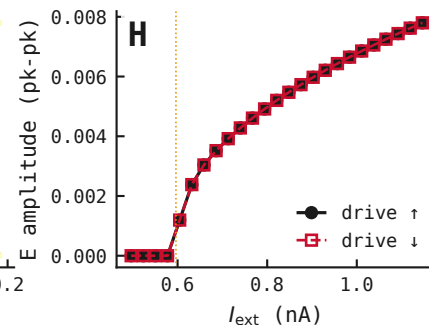
Supercritical, reversible onset
