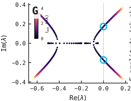
Hopf crossing at I^* = 0.60 nA
