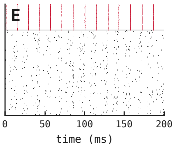
W EI =0.6, W IE =1.2 contrast=0.27
