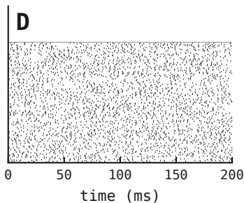
W EI =0.0, W IE =0.0 contrast=0.00
