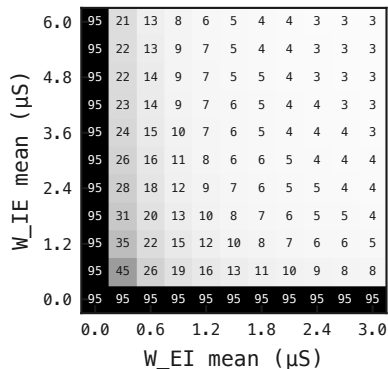
E firing rate (Hz)
