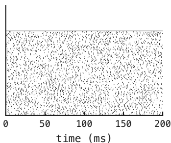
A W_{EI}=0.0 , W_{IE}=3.6 contrast=0.00
