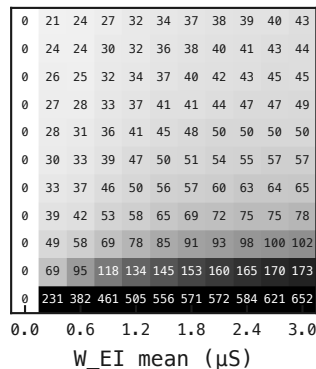
I firing rate (Hz; edge clipped)
