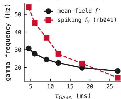
Frequency from biophysics
