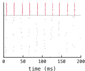
C W_{EI}=3.0 , W_{IE}=6.0 contrast=0.96
