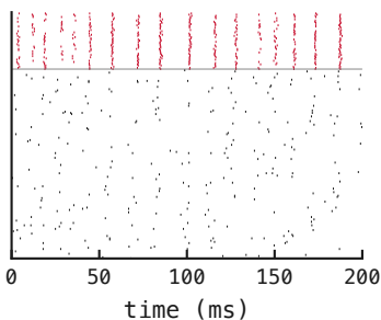
B W_{EI}=1.2 , W_{IE}=2.4 contrast=0.45
