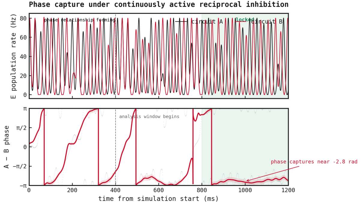
Figure 1: Phase capture during the first 1.2 s of the strength 0.2, intermediate-delay condition. Reciprocal coupling is active from the first timestep. The two population rhythms initially have an unstable relative phase; their circular phase difference then concentrates near -2.8 rad. This is phase locking, not zero-lag synchrony. The dashed line marks the registered transient exclusion and the green band highlights the capture interval. Full-window metrics and later phase slips remain included in the registered analysis.
