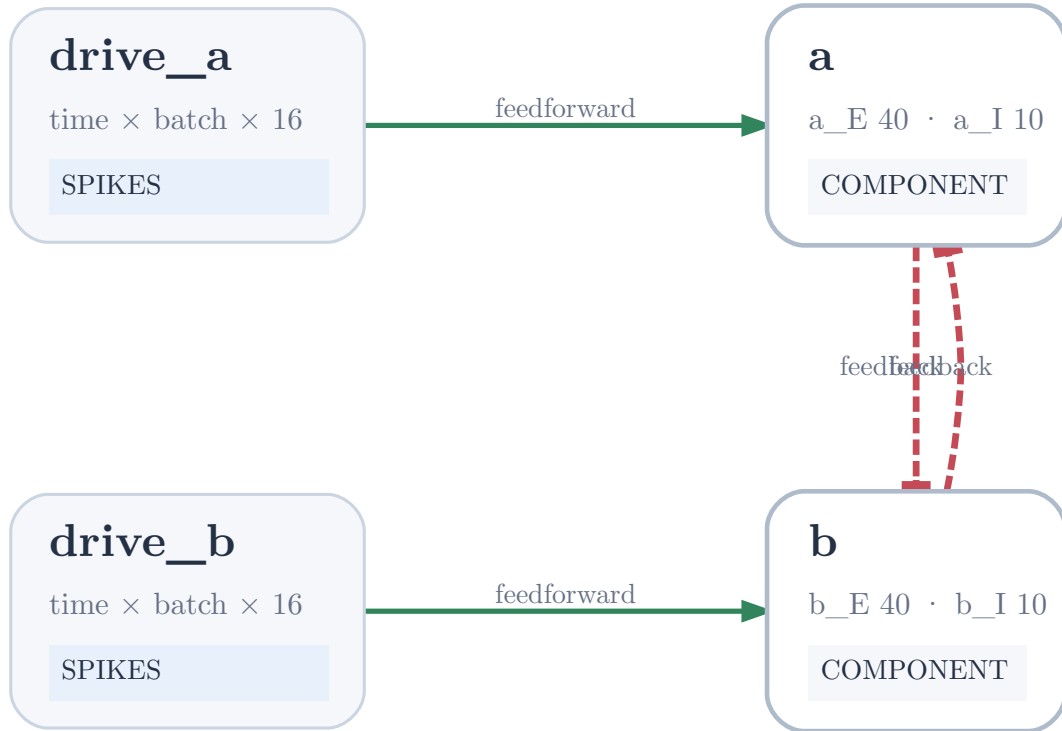
Figure 2: Representative reciprocal graph. Each inhibitory population sends a delayed GABA projection to the other circuit’s excitatory population; the two input nodes are independent.
