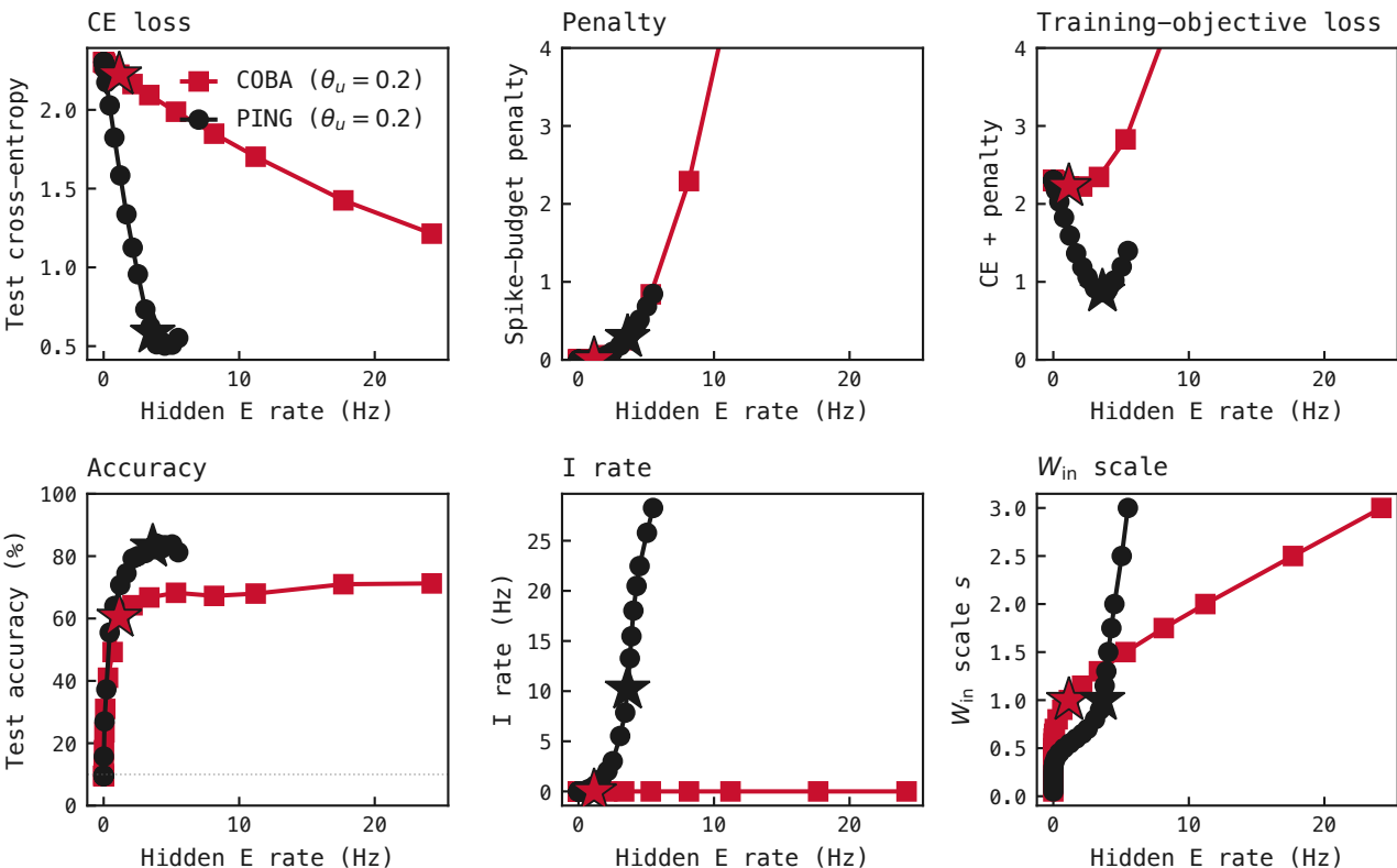
Inference-time W_{in} scale sweep — replotted vs E rate (stars mark trained s=1 )
