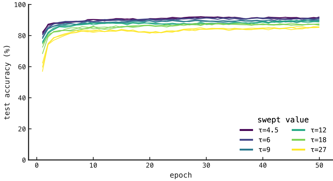
Figure 15: Test accuracy over epochs across the \tau _GABA ladder; cells converge to similar accuracy regardless of inhibitory decay.
