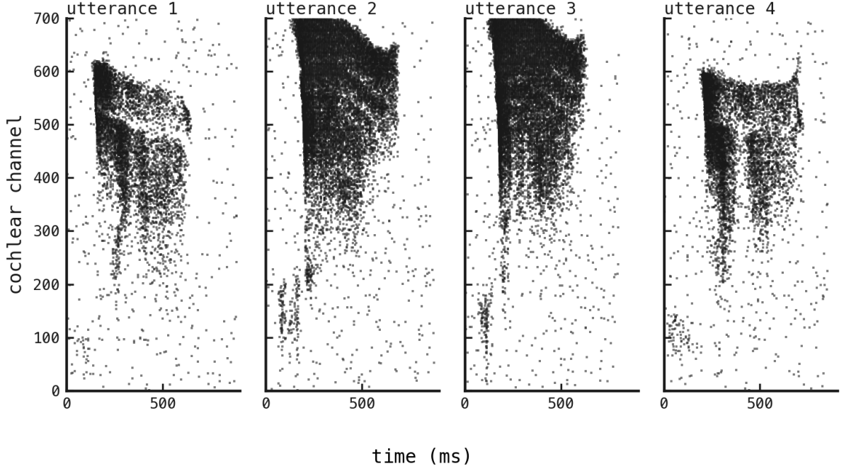
Figure 116: 4 different utterances of class 0, null , each a raster of time (ms) against cochlear channel: the within-class spread. What we expect. Different speakers saying the same word should share a family resemblance while differing in the particulars. What we see. Exactly that: all 4 carry the same broad high-channel onset falling into a mid-channel body, but they differ in duration, event density, and the fine structure of the low-channel tail. This speaker variability is what a classifier trained on SHD must generalise over.
