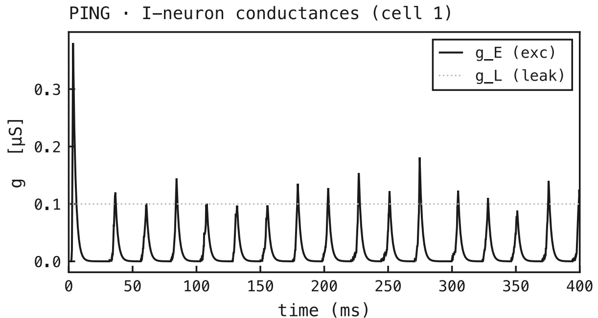
Figure 56: Conductances on the I cell, PING mode. The I cell receives only excitation : g_E (black) is the arriving E-spike envelope (delivered via W_{ei} ) and g_L (faint) is the fixed leak. There is no inhibitory conductance — the architecture has no I→I synapse — which is exactly why the I population can synchronise into the sharp once-per-cycle bursts that clock the loop.
