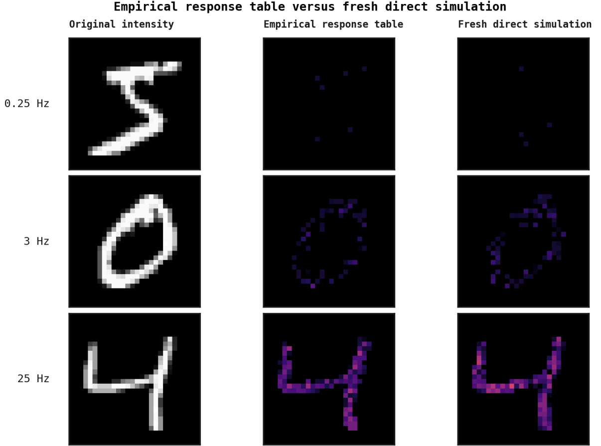
Figure 131: Training-image feature comparison. Rows show an original MNIST training image, a response-table sample, and a fresh direct simulation at 0.25, 3, and 25 Hz for the nominal 1.2 \mu S probe, using common 0–65 mV limits. Increasing rate reveals the intensity pattern as spatial signal grows relative to independent sampling noise.
