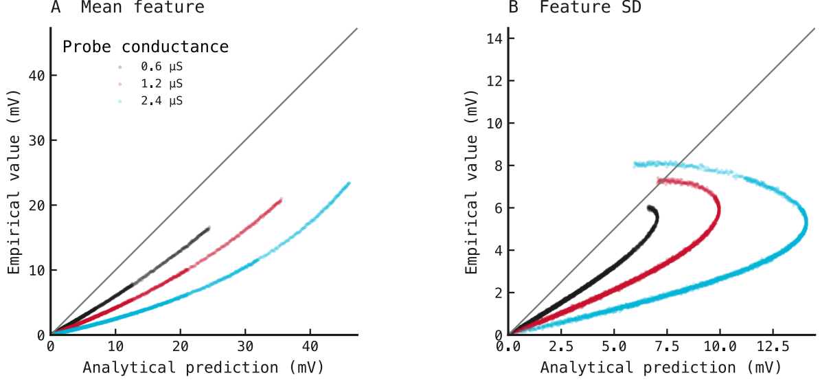
Figure 130: Operating-point linearized predictions versus empirical response moments. Each point is one rate–intensity condition; colour denotes probe conductance, and empirical moments pool draws across three seeds. Panel A compares the predicted mean of z from Equation 12a ( \mu_{\text{linear}(z)} ) with the empirical mean of z . Panel B compares the predicted SD of z , \sqrt{\text{Var}_{\text{linear}(z)}} from Equation 18, with the empirical SD of z . The diagonal marks equality. Mean ordering is preserved (Pearson r = 0.951 ), but the median prediction is 2.52-fold larger. SD agreement is weaker ( r = 0.741 ), with median 2.245-fold overprediction. Points lie mainly below equality because the stationary linearization omits the start-from-rest transient, finite-window nonstationarity, discrete input, and conductance fluctuations.
