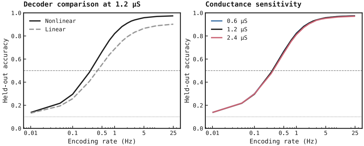
Figure 133: Official-test psychometric curves. Each point pools the official 10,000-image test partition across three fresh simulation draws and three independently trained runs. Within each rate, conductance, and draw, runs share feature vectors; different conductances use different spike draws. Accuracies, not predictions, are averaged. Bands bootstrap images, draws, and runs; horizontal rules mark 10% uniform guessing and the 50% pragmatic criterion. Accuracy rises as more pixels spike within 200 ms. Because each conductance has separately retrained decoders, overlap shows recoverability after retraining, not robustness of one fixed decoder.
