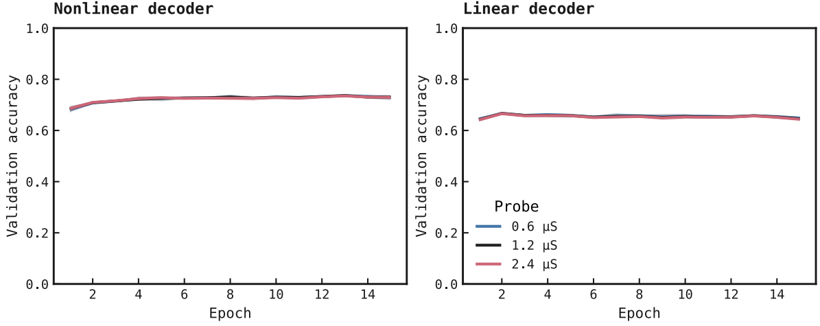
Figure 132: Mixed-rate validation histories. Each panel plots mean validation accuracy across decoder seeds, with their range shaded, under equal sampling of all 15 rates from 0.01–25 Hz and fresh direct simulations. Curves rise then flatten as class structure is acquired; conductances overlap because response scaling preserves similar spatial evidence.
