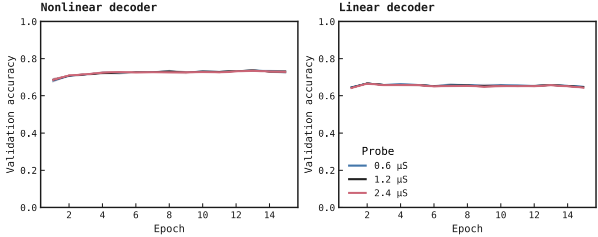
Figure 8: Mixed-rate validation histories. Each panel plots mean validation accuracy across decoder seeds, with their range shaded, under equal sampling of all 15 rates from 0.01–25 Hz and fresh direct simulations. Curves rise then flatten as class structure is acquired; conductances overlap because response scaling preserves similar spatial evidence.
