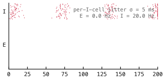
Smear bursts → E rate falls to zero
