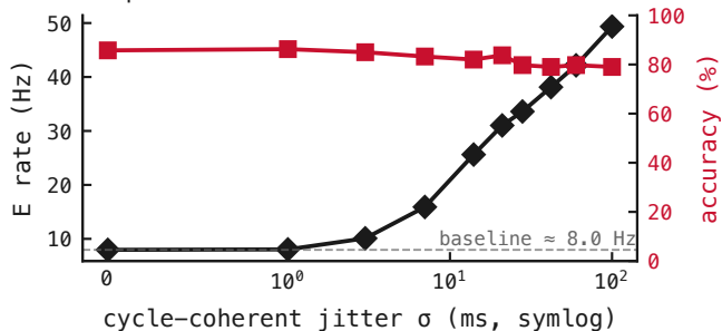
Displace bursts → E rate rises
