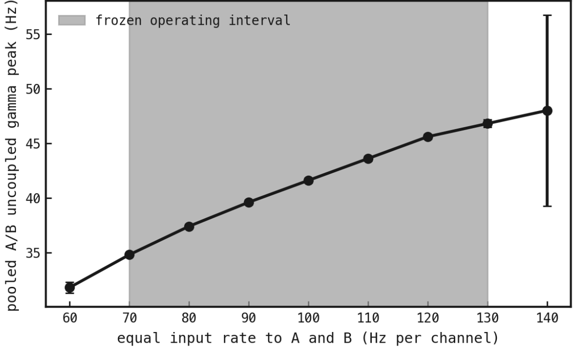
Figure 2: Uncoupled input-rate calibration. Circuits A and B receive the same input rate, shown in hertz per channel on the horizontal axis. At each rate, the vertical coordinate is the median of 10 gamma-peak estimates: both circuits from each of five trials. Bars show half the interquartile range of those pooled A/B estimates, spanning the middle half of the data. The shaded 70–130 Hz interval supplies Equation 1. The lowest-rate point exceeds the registered within-rate IQR ceiling. At the highest rate, the estimator hops between two separated spectral modes across seeds, producing the large bar. Both boundary conditions are excluded.
