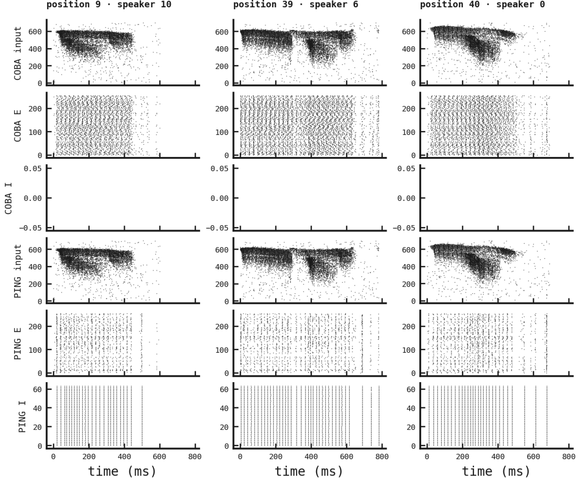
Figure 2: Matched validation rasters for candidate 1. Each COBA/PING column uses byte-identical binned input and fixed validation positions.
