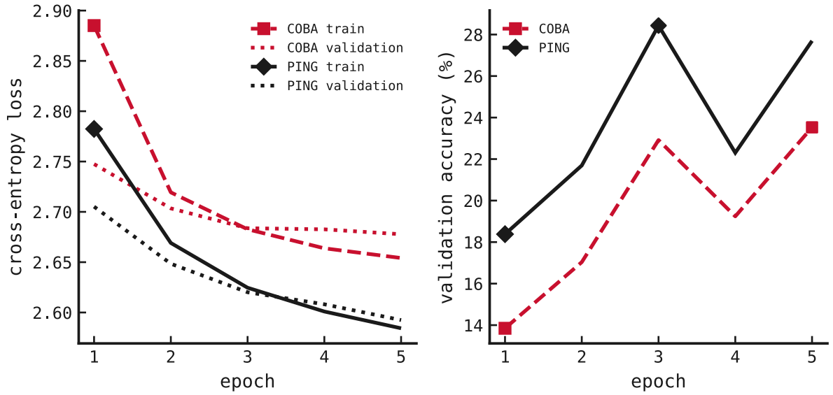
Figure 1: Candidate 1 learning curves. The registered decision uses epoch five, not the visually best intermediate checkpoint. Candidate-specific curves for all three attempts are retained in the artifact bundle.
