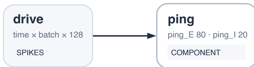
Figure 120: Compiled SNNLANG graph at the 9 ms default condition. Across the sweep, only the decay time attached to the I-to-E GABA projection changes. The input tensor, populations, weights, delays, and execution seeds are paired across conditions.
