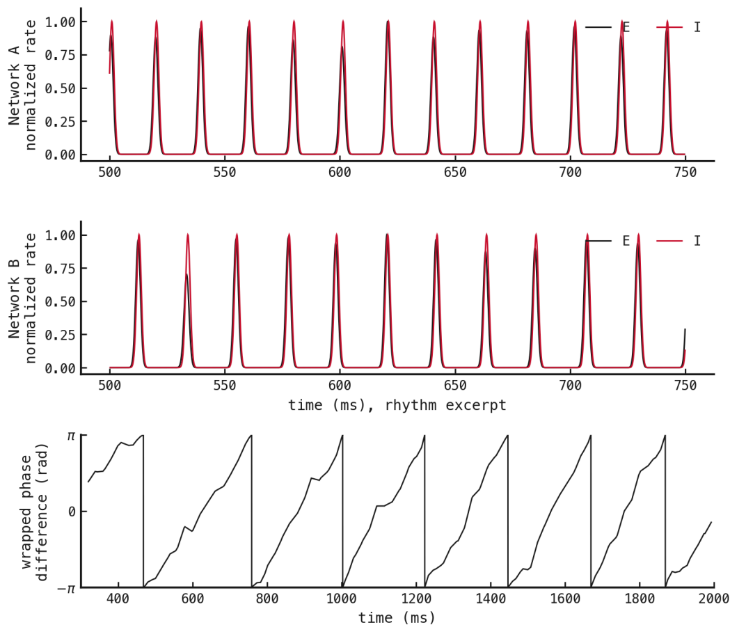
Figure 124: Both networks sustain gamma rhythms, but their relative phase keeps moving.
