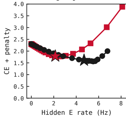
Training-objective loss
