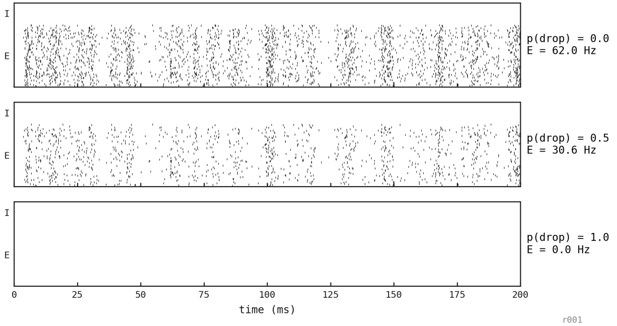
Figure 4: Illustrative seed-42 COBA replayed across the same drop sweep. With no cycle to preserve, dropping spikes just thins a uniform asynchronous mean.
