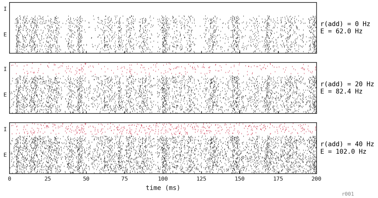
Figure 5: Illustrative seed-42 COBA replayed across the same add sweep. Added spikes blend into COBA's asynchronous mean: no temporal structure to corrupt, just a higher mean rate.
