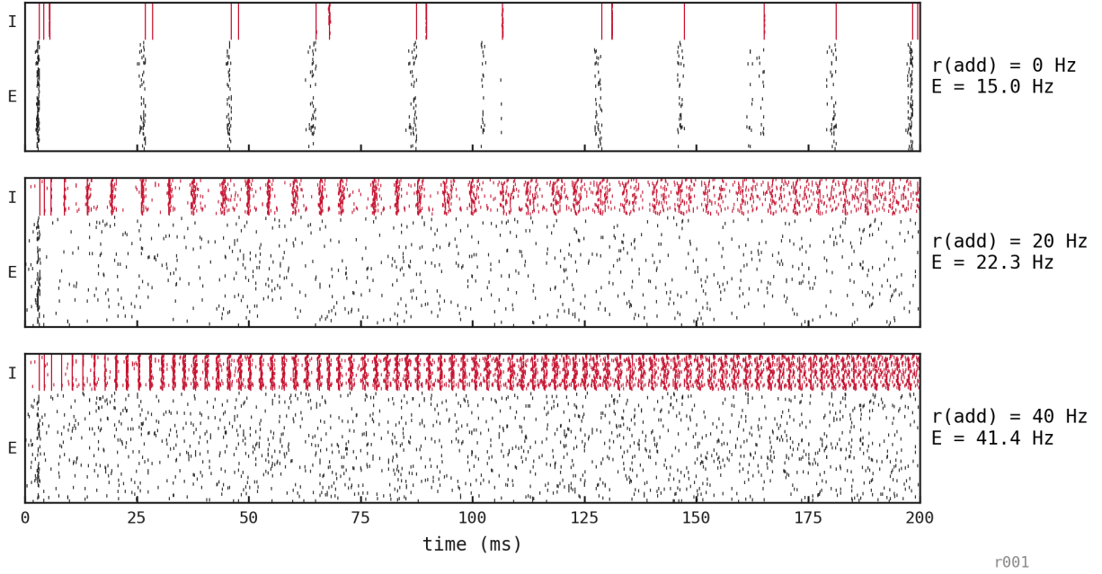
Figure 3: Illustrative seed-42 PING replayed across three added-noise levels (0, 20, 40 Hz per neuron). The gamma banding dissolves into asynchronous firing as the added rate rises, matching the accuracy cliff in the previous figure.
