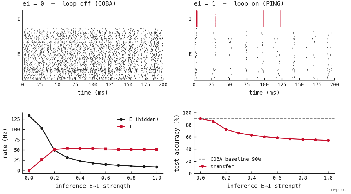
Figure 1: Switching the recurrent I-loop on at inference on a trained COBA network (no retraining; W^{EI}/W^{IE} freshly wired, since the COBA checkpoint stores them at zero). Top : the same feedforward weights fire densely and asynchronously at ei = 0 (COBA) and in gamma bands at ei = 1 (PING); the gamma dynamics come from the inhibitory architecture, not from training. Bottom left : E rate falls \approx 15\times ( \approx 133 \rightarrow 9 Hz) as the loop engages while I rises to \approx 51 Hz; the suppression is continuous in loop strength. Bottom right : accuracy degrades without retraining, from the \approx 90\% COBA baseline to \approx 55\% at full strength (a \approx 36 pp cost). So the architecture supplies the rate-gating for free, but using it well needs training with the loop (exp025): the sparsity is architectural, the accuracy is learned.
