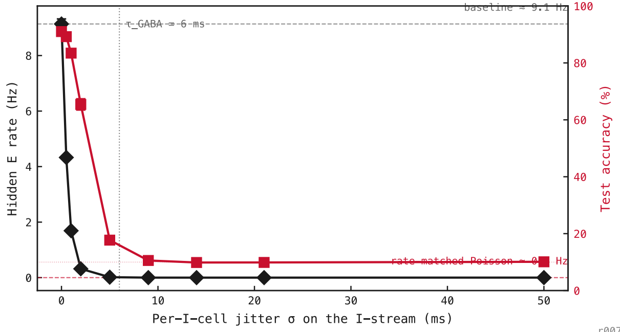
Figure 2: Per-I-cell jitter sweep, three seeds. Each spike receives an independent Gaussian offset; mean per-cell I rate is preserved exactly. E rate (black diamonds, left axis) falls monotonically from baseline (9.1 Hz) , already more than halved to 4.3 Hz by \sigma = 0.5 ms and essentially zero (0 Hz) by \sigma \approx 5 ms, below \tau_{\text{GABA}} = 6 ms. Accuracy (red squares, right axis) holds at \approx 89.2\% up to \sigma = 0.5 ms , then collapses through 83.4% ( \sigma = 1 ), 65.4% ( \sigma = 2 ) and 17.7% ( \sigma = 5 ), bottoming at chance (10.6%) by \sigma = 9 ms. The \sigma \rightarrow \infty asymptote is the rate-matched Poisson regime: E silent, accuracy at chance.
