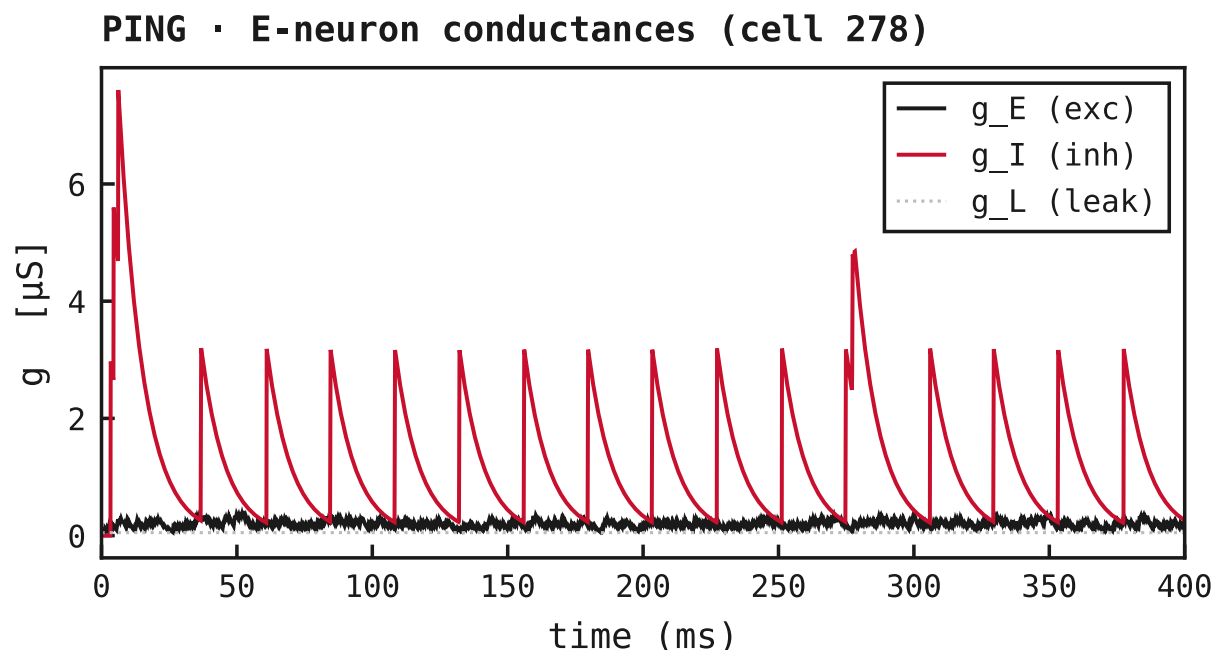
Figure 40: Conductances on the same E cell, PING mode. The inhibitory conductance g_I (red) now dominates — it spikes once per gamma cycle as the synchronous I-burst arrives through W_{ie} , then decays with \tau_{\text{GABA}} — while g_E (black) carries the smaller feedforward input and g_L (faint) is fixed. All three traces are non-negative : g_I is large and positive, and that is what shunts the cell — it carries no sign of its own.
