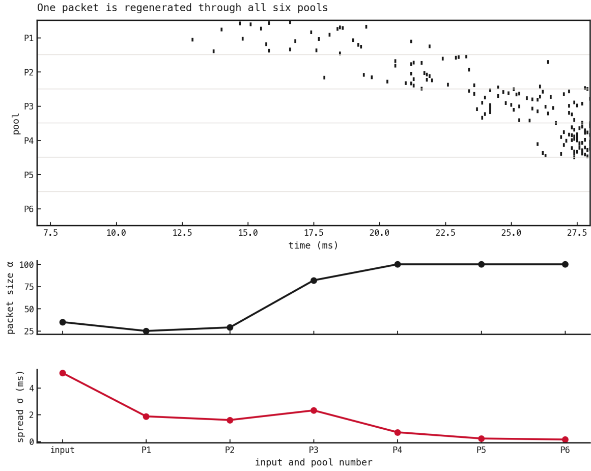
Figure 6: Reference-packet propagation at total feedforward strength 0.22 \mu\text{S} and background rate 30 Hz.
