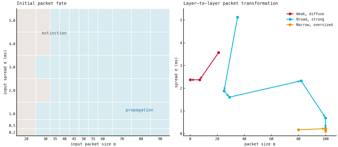
Figure 8: Measured packet state space. Tiles classify 77 initial size-width combinations. Arrows follow the three representative packets from their inputs through successive pools. 67 of 77 tested packets reach Pool 6. The boundary shifts toward larger \alpha as \sigma increases: temporally diffuse packets require more spikes. Surviving trajectories collapse toward the saturated 100-spike state, while the weak trajectory moves toward extinction.
