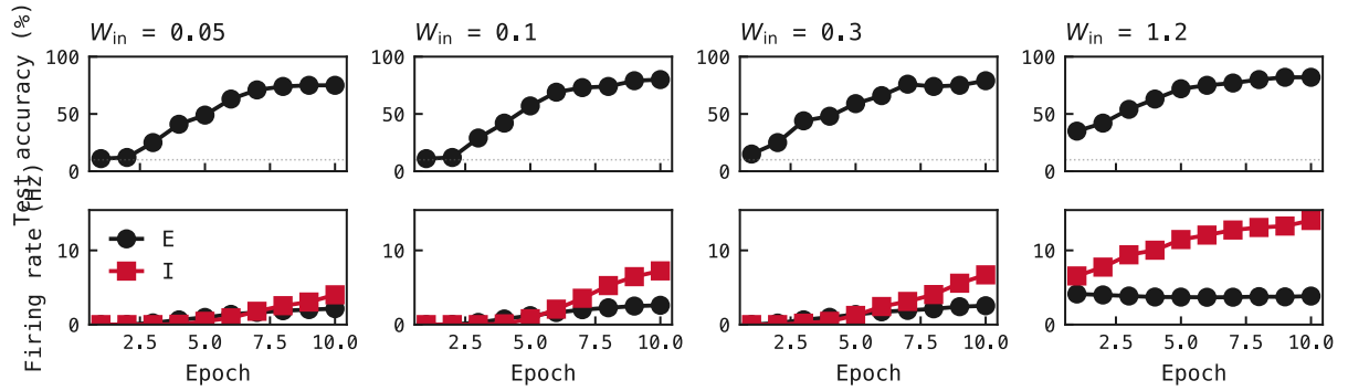
Figure 72: Per-epoch training traces from four PING networks (seed 42, \theta_u = 0.2 from epoch 0), one per column. Top: test accuracy. Bottom: test-set E (black) and I (red) firing rates. At W_{in} = 0.05 and 0.1 the I population is silent for the first one to two epochs; once W_{in} crosses the recruitment threshold the loop engages and the network locks into PING. Final accuracies: 84.0% / 84.5% / 85.0% / 83.75%; final I rates: 11.1 / 15.5 / 6.9 / 16.7 Hz.
