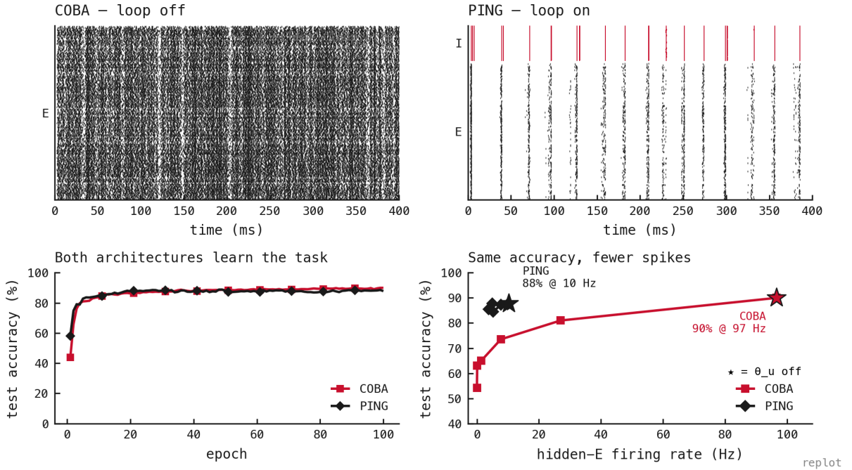
Figure 70: The headline comparison in one 2 \times 2 frame (rasters, learning, and the accuracy–rate frontier together). Top — trained-baseline single-trial rasters on the same MNIST digit 0 input: COBA ( –ei-strength 0 ) fires densely and asynchronously at \approx 97 Hz (I silent, loop off); PING ( –ei-strength 1 ) fires in gamma bands at \approx 28 ms cadence ( \approx 10 Hz per E cell) with synchronous I bursts (red) above E (black). Same architecture, parameter count, and recipe — only PING’s recurrent E \leftrightarrow I matrices are non-zero. Bottom left — test accuracy per epoch (mean over three seeds): both reach \approx 88\% , so both learn the task. Bottom right — the accuracy–rate frontier across the spike-budget penalty \theta_u : PING sits up-and-left of COBA — the same accuracy at a fraction of the hidden-E rate — with the \theta_u -off operating points starred and labelled (PING 88% at \approx 10 Hz, COBA 90% at \approx 97 Hz). COBA red, PING black; E black / I red in the rasters. The headline of this entry: gamma gating buys an order-of-magnitude per-spike economy at matched accuracy.
