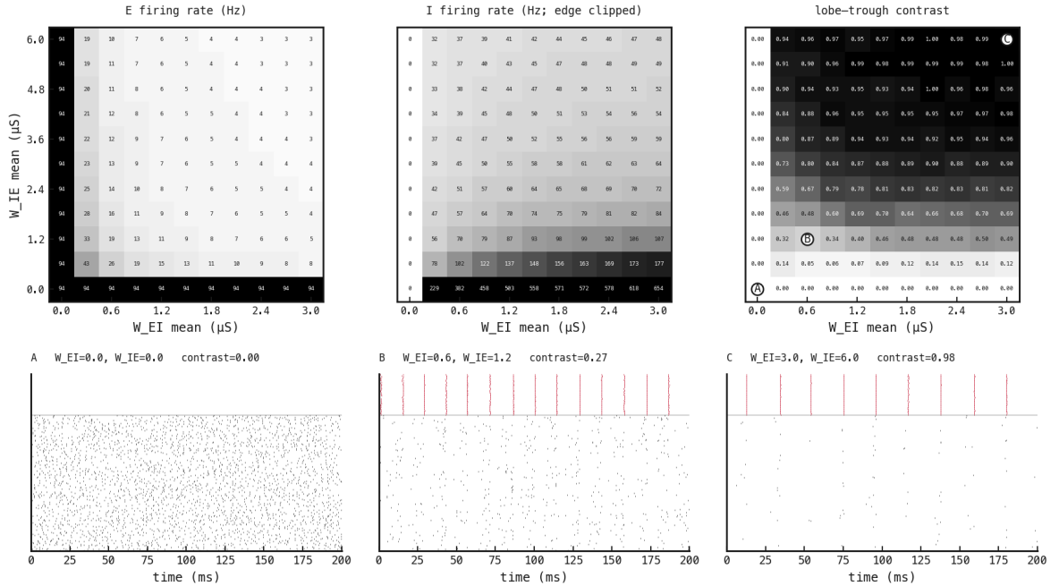
Figure 163: The anchor result: gamma switches on smoothly across the recurrent-weight plane, read as scalar maps over the W_{EI} \times W_{IE} grid (untrained networks, private per-cell Poisson input) with example rasters beneath. Top — three per-cell summaries, every cell labelled. E rate is high along both zero edges (the loop is broken, E fires at the input-driven \approx 95 Hz) and gated down through the interior; I rate is silent where W_{EI} = 0 , runs away along W_{IE} = 0 (clipped so the interior is legible), and is controlled once the loop closes; lobe–trough contrast (the rhythm scored 0–1) reads exactly 0 along both COBA edges and rises smoothly toward strong coupling, with three points marked along the W_{IE} = 2W_{EI} diagonal. Bottom — E/I rasters (E black, I red above) at those points: A the fully-off origin ( W_{EI} = W_{IE} = 0 ), asynchronous with no I; B weak coupling, emerging volleys (contrast 0.27, below the half-way mark); C strong coupling, sharp volleys (contrast 0.98). E rate falling, I rate rising, and contrast rising are three readings of the same loop engaging. The full per-cell detail — every raster and autocorrelogram — is in the figures below; the rate-fairness behind the contrast metric is in Figures 4–5.
