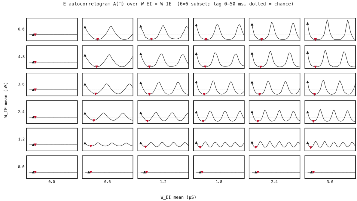
Figure 165: The E-population autocorrelogram A(\ell) for a 6×6 subset of the grid (lag 0–50 ms; dotted line = chance, A = 1 ), with the located lobe (▲) and trough (▼) marked. The two zero edges are flat at 1 — asynchronous firing, no structure. Through the interior the Mexican hat emerges: a sharp central lobe at \approx 1 ms over a trough near the half-period, with a secondary peak at the full period further out. The contrast in Figure 1 is exactly this lobe-versus-trough read off as one number.
