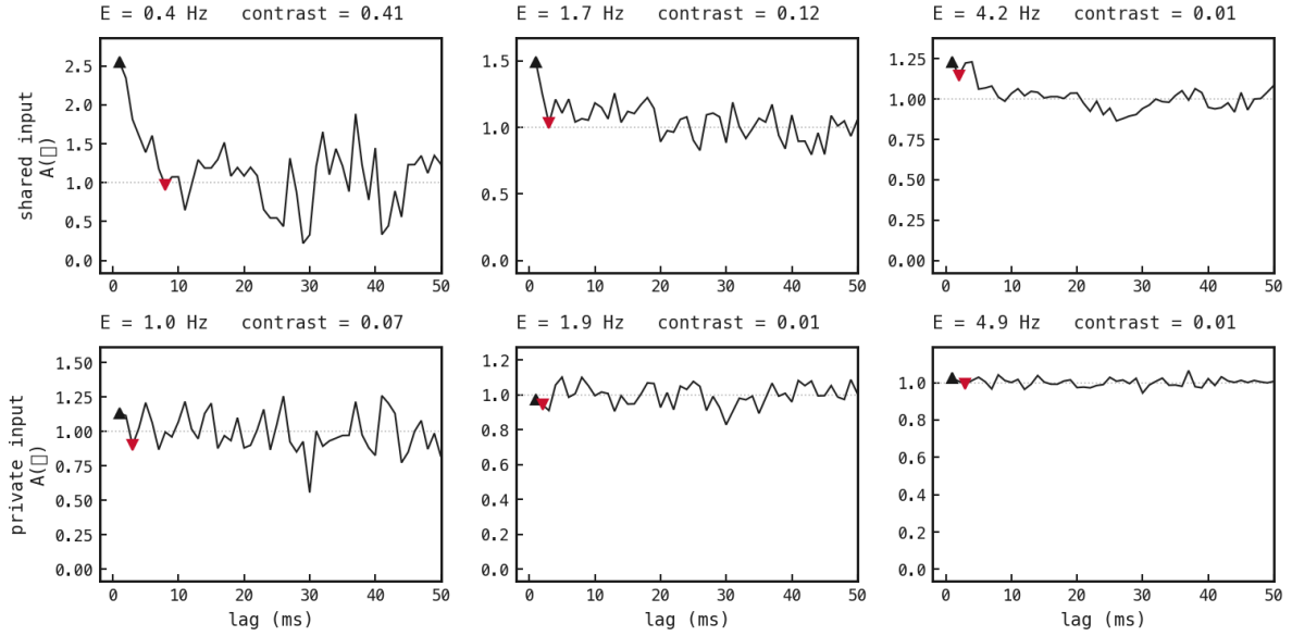
Figure 167: Why shared input fails and private input does not, at matched low firing rates. Top (shared input): coincident spikes from shared channels leave a central peak over a shallow dip — a spurious hat with no inhibitory loop behind it — and the metric marks a lobe ( \blacktriangle ) and trough ( \blacktriangledown ) and reports a non-zero contrast. Bottom (private input): the same firing rates, but with one channel per cell the central peak is gone; A(\ell) is flat shot-noise around chance and the contrast collapses to \approx 0 . Same rate, same spike counts — the only difference is whether cells share input.
