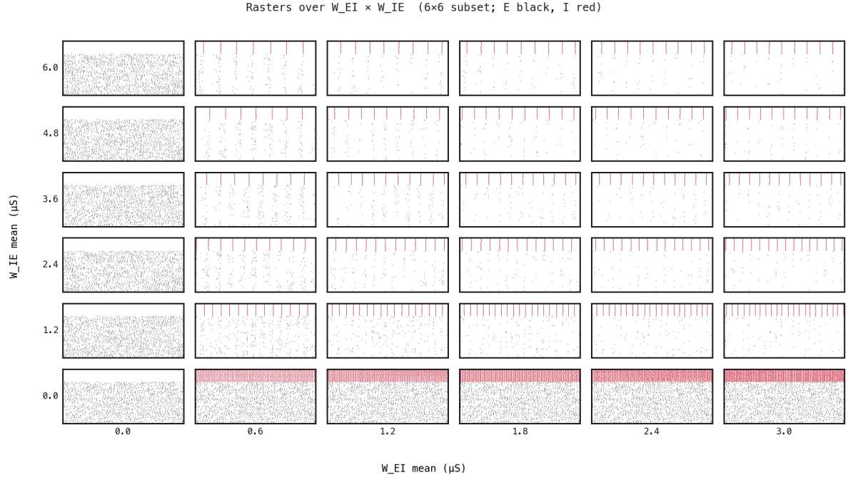
Figure 164: E/I rasters for a 6×6 subset of the grid (every other cell; the heatmaps below use all 121). The two zero edges are the controls: W_{EI} = 0 (left column) leaves I silent and E asynchronous; W_{IE} = 0 (bottom row) lets I fire but not inhibit E, so both stay dense — neither is rhythmic. The interior shows clear gamma volleys (E black, I red) that sharpen as either weight grows — the rhythm the contrast (Figure 1) scores.
