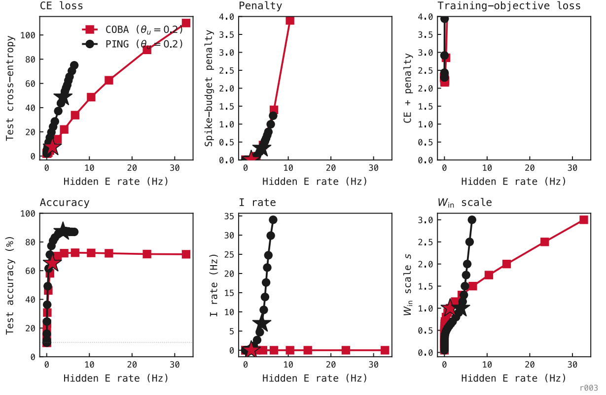
Figure 5: The same 24-point sweep as Figure 4, re-projected with hidden E rate on the x-axis. Filled stars mark each cell's trained operating point ( s = 1 ): PING at E \approx 3.8 Hz, COBA at E \approx 1.3 Hz. PING's accuracy reaches its plateau ( \approx 88\% ) just past its trained operating point; COBA climbs slowly and only reaches \approx 71\% even at E \approx 33 Hz.
