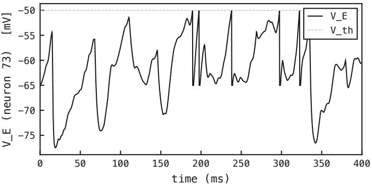
PING · E-neuron membrane voltage
