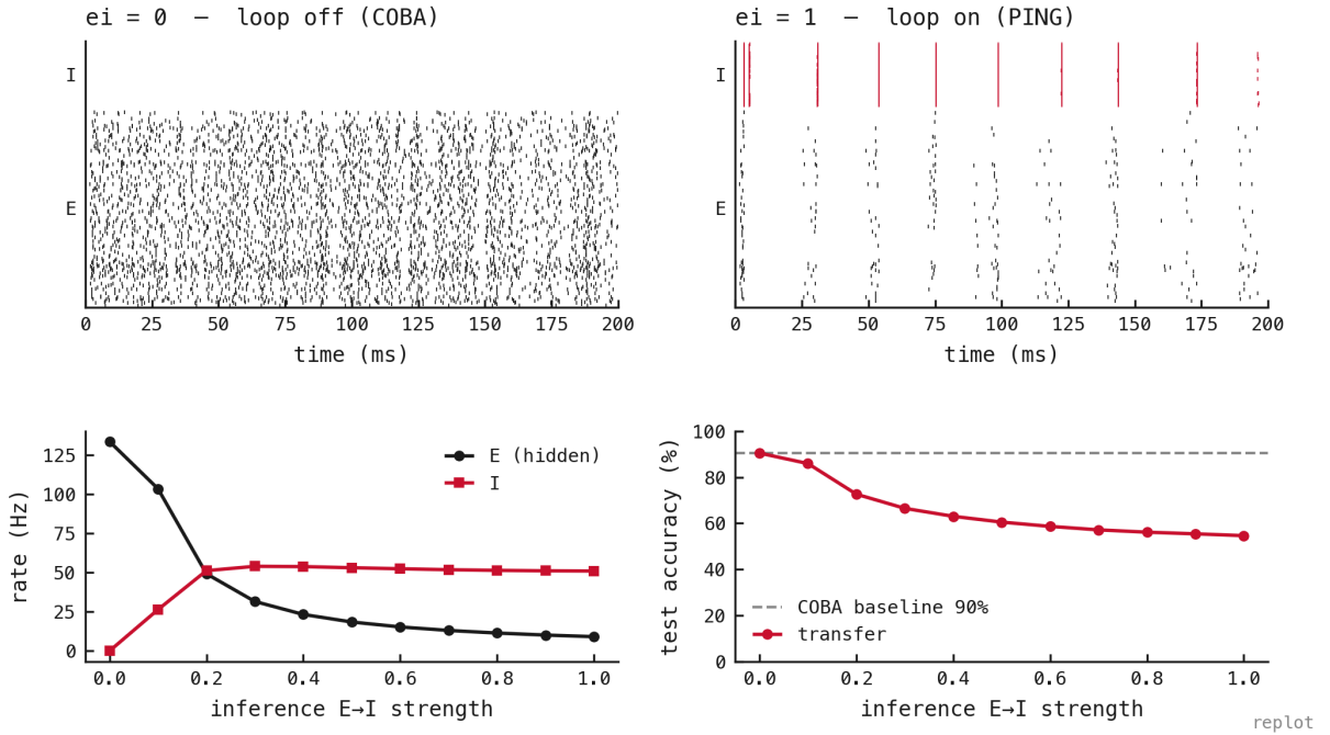
Figure 4: Engaging the recurrent loop at inference reproduces the PING firing-rate reduction with no weight update. COBA networks trained with seeds 42–44 are evaluated with recurrent E \rightarrow I coupling scaled from ei = 0 to ei = 1 , without retraining. Top: illustrative seed-42 rasters at loop-off and full strength. Bottom left: across-seed mean excitatory (black) and inhibitory (red) rates; excitation falls approximately 15-fold (from \approx 133 to \approx 9 Hz) as inhibition rises to \approx 51 Hz. Bottom right: mean accuracy falls from \approx 90\% to \approx 55\% (a \approx 36 pp cost). Shaded bands show sample SD across seeds. The rate gating appears when the loop is wired in, whereas the accuracy loss reflects the absence of a feedforward compensation learned in the presence of the loop. Source: exp038.
