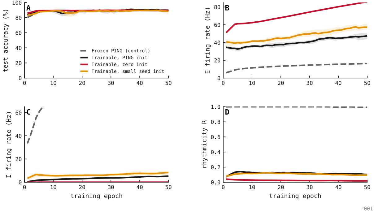
Figure 5: Releasing the loop weights to gradient descent prunes the rhythm within a single epoch, from every initialisation. Per-epoch training metrics with the recurrent weights W^{EI} , W^{IE} made trainable under the Dale’s-law clamp, over 50 epochs on MNIST. Lines are the mean of three seeds (42–44); shading is the across-seed range. Conditions differ only in initialisation of the loop weights: canonical PING values (black), zero (red), and 0.1 \times canonical (amber), against a frozen-PING control (grey, dashed). (A) Test accuracy: all conditions overlap at \approx 84 – 91\% . (B) Mean excitatory firing rate: the trainable conditions rise to \approx 49 – 88 Hz as the loop is dismantled, while the frozen control remains gated near 17 Hz. (C) Mean inhibitory firing rate: the trainable conditions collapse to \approx 0 Hz within a few epochs, while the frozen control’s inhibitory rate rises to \approx 108 Hz as its readout trains. (D) Lobe–trough rhythmicity contrast: the frozen control holds at \approx 1 while every trainable initialisation drains to \approx 0.02 – 0.11 . Source: exp049.
