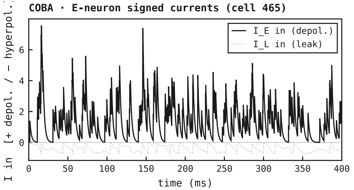
Figure 4: Signed synaptic currents into the E cell, COBA mode, with I_X^{in} = -g_X(V - E_X) (positive = depolarising). With no inhibition, the only synaptic current is the depolarising excitatory current I_E^{in} (black); the leak current (faint) hovers near zero. Compare Figure 3c, where the loop introduces an inhibitory current of the opposite sign.
