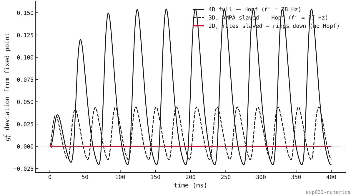
Figure 9: The reductions tested by simulation: g_e^F after a small kick at a common drive ( I_{\text{ext}} = 1 nA, above every threshold). The 4D model (black, f^* = 28 Hz) and the 3D AMPA-slaved reduction (black dashed, f^* = 37 Hz) both sustain the limit cycle; the 2D rate-slaved reduction (red) rings down to its fixed point: no Hopf, as eq (35) requires.
