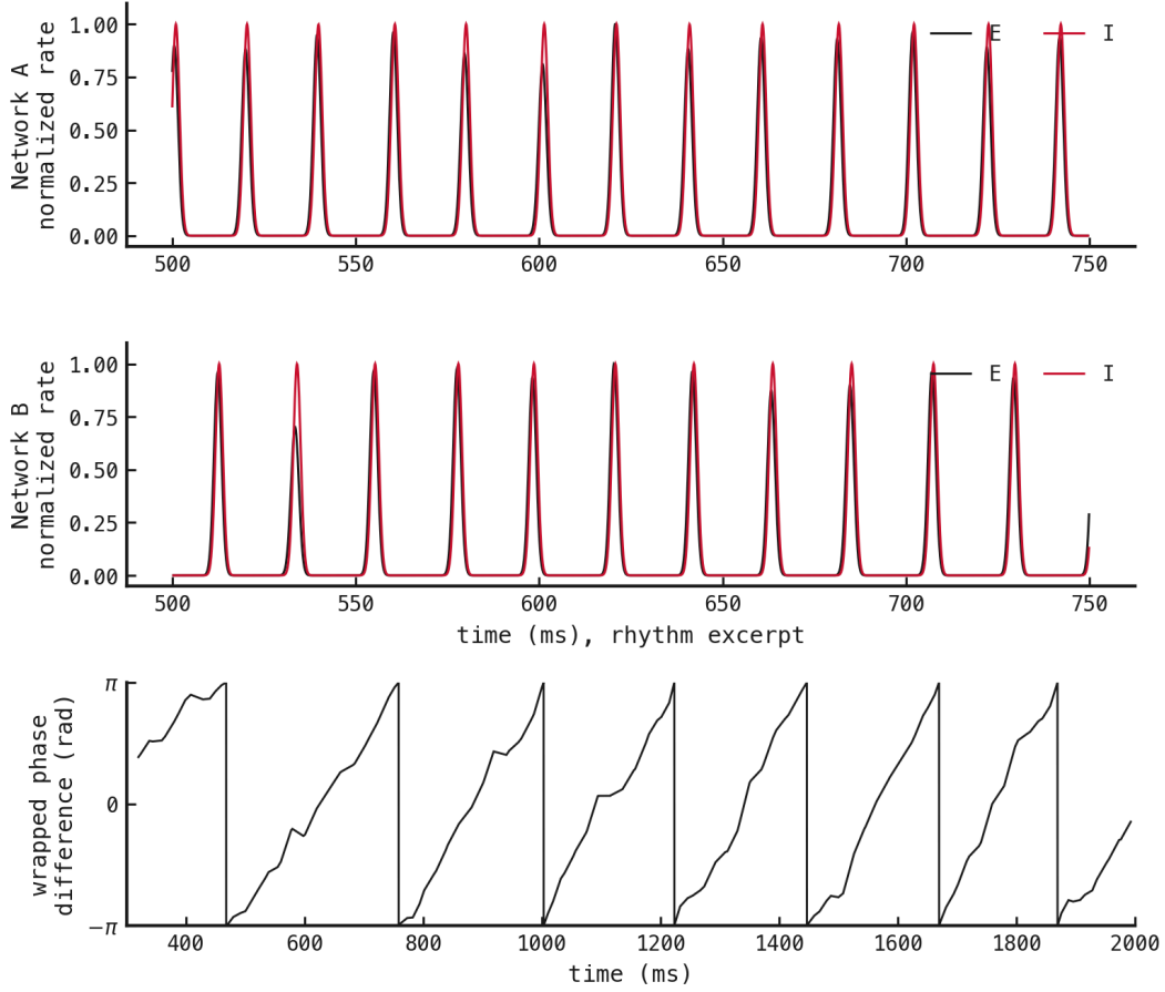
Figure 2: Both networks sustain gamma rhythms, but their relative phase keeps moving. Network A oscillates at 50.7 Hz and Network B at 46.7 Hz. Their low interval variability confirms regular rhythms. Relative phase wraps 7 times, establishing the drift that coupling must stop.
