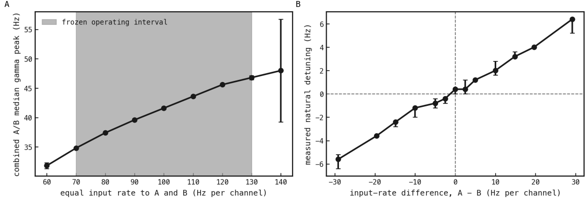
Figure 120: Calibration of frequency and natural detuning. (A) Circuits A and B receive the same input rate. Each point is the median of 10 gamma-peak estimates: both circuits from each of five trials. Bars show half the interquartile range of the combined estimates. The shaded 70–130 Hz interval supplies the rate pairs used in Equation 1. The lowest-rate point exceeds the registered within-rate IQR ceiling. At the highest rate, the estimator hops between two separated spectral modes across seeds, producing the large bar. Both boundary conditions are excluded. (B) The circuits remain uncoupled but receive unequal input rates. The horizontal axis is the A-minus-B input-rate difference; the vertical axis is the median natural detuning from Equation 1 across five paired seeds. Bars span the interquartile range; dashed lines mark zero drive difference and zero detuning.
