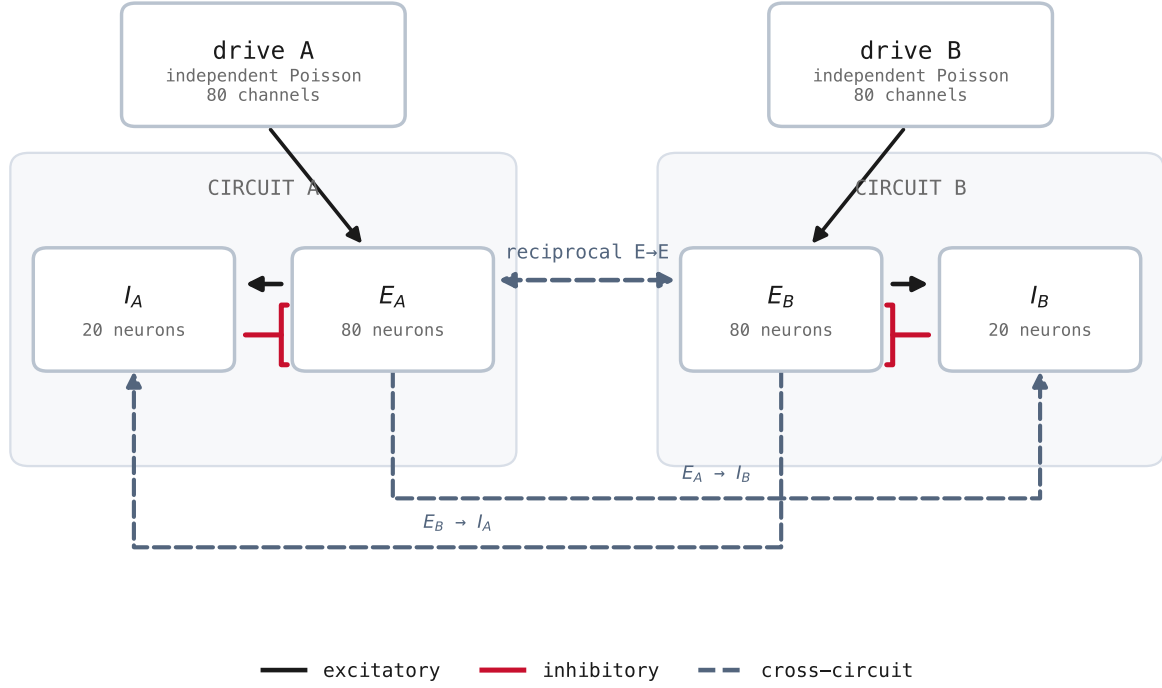
Figure 1: Two-circuit coupling intervention. Each private Poisson input drives a local E-to-I-to-E PING loop. Dashed pathways are the four reciprocal AMPA projections varied together by coupling weight K ; red bar-headed pathways are local GABA-A inhibition. Only the dashed pathways vary across the primary grid.
