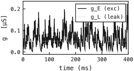
C0BA – no recurrent loop (ei-strength = 0) – E-neuron conductances (cell 334)
