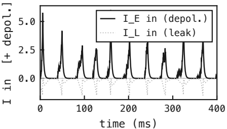
PING – recurrent loop active (ei-strength = 1.5) – I-neuron signed currents (cell 3)
