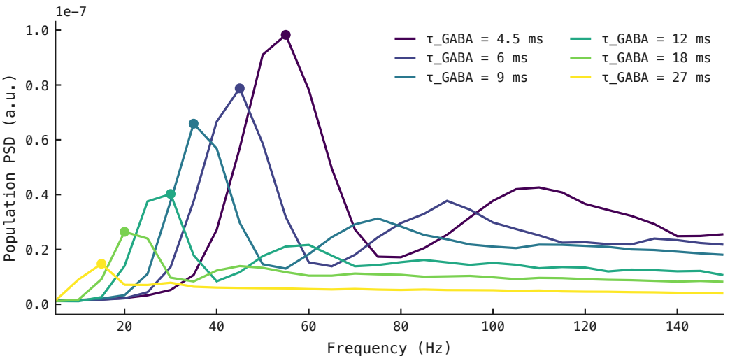
Trained-network population PSDs — peak marks f_\gamma
