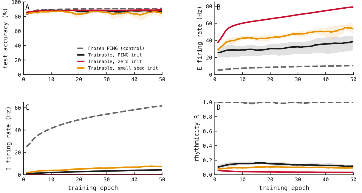
Figure 5: Releasing the loop weights to gradient descent prunes the rhythm within a single epoch, from every initialisation. Per-epoch training metrics with the recurrent weights W^{EI}, W^{IE} made trainable under the Dale’s-law clamp, over 50 epochs on MNIST. Lines are the mean of three seeds (42–44); shading is the across-seed range. Conditions differ only in initialisation of the loop weights: canonical PING values (black), zero (red), and 0.1 \times canonical (amber), against a frozen-PING control (grey, dashed). (A) Test accuracy: all conditions overlap at \approx 90 – 92\% . (B) Mean excitatory firing rate: the trainable conditions rise to \approx 37 – 76 Hz as the loop is dismantled, while the frozen control remains gated near 10 Hz. (C) Mean inhibitory firing rate: the trainable conditions collapse to \approx 0 Hz within a few epochs, while the frozen control’s inhibitory rate rises to \approx 57 Hz as its readout trains. (D) Lobe–trough rhythmicity contrast: the frozen control holds at \approx 1 while every trainable initialisation drains to \approx 0.03 – 0.14 . Source: exp049.
